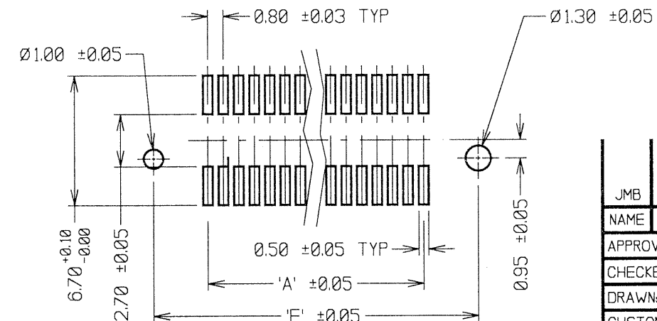
RECOMMENDED PAD LAYOUT
