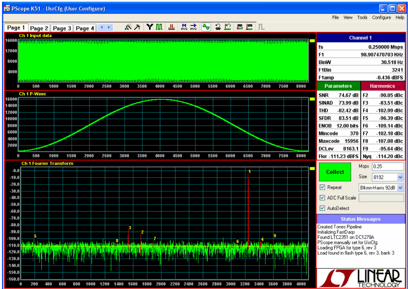
Figure 2. SOFTWARE SCREENSHOT
