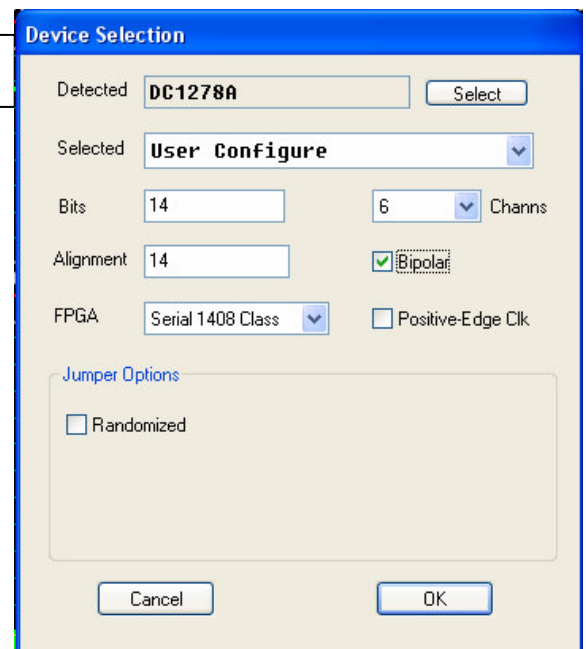
Figure 3. CONFIGURE MENUS
