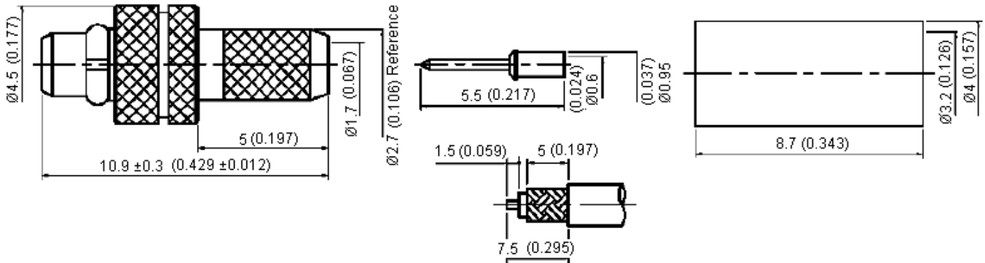
Stripping Dimension
