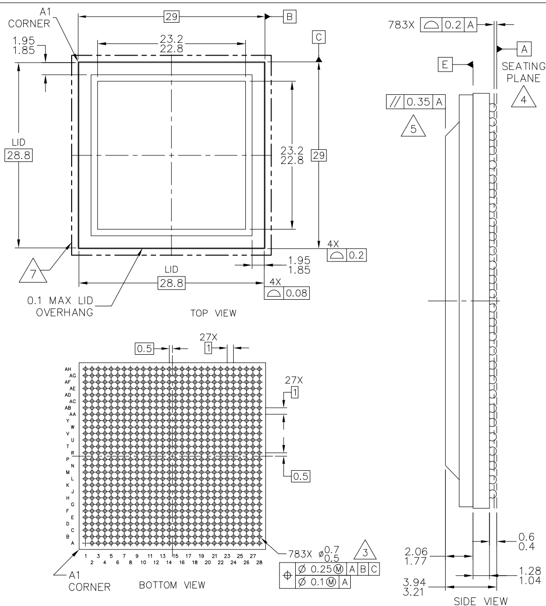
Figure 31. MSC8157 Mechanical Information, 783-ball FC-PBGA Package
