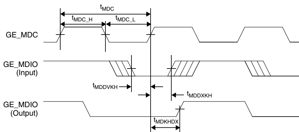
Figure 22. MII Management Interface Timing
