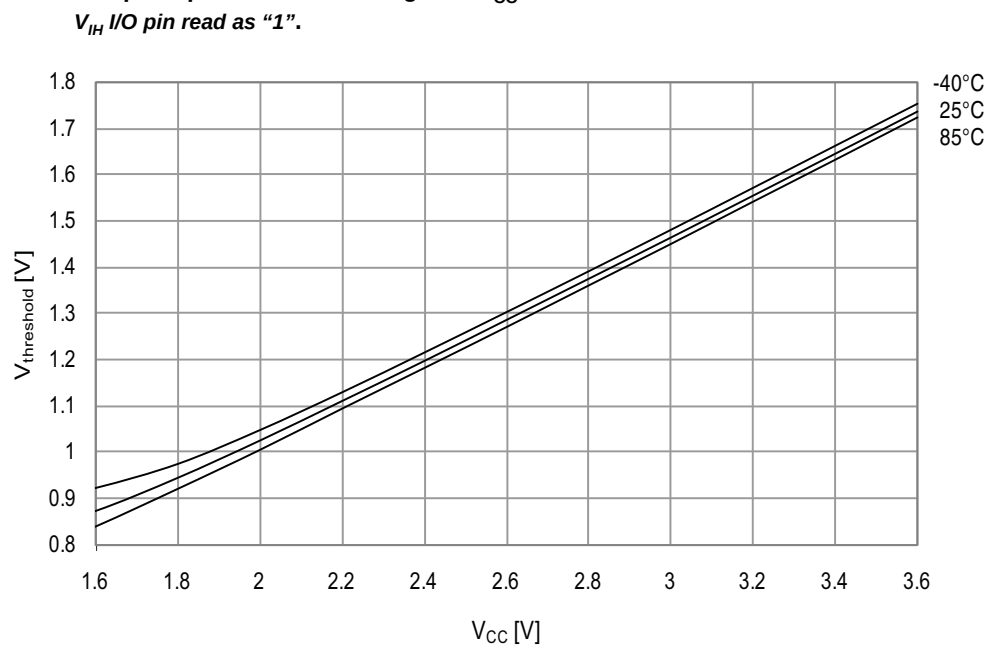
Figure 34-96. I/O pin input threshold voltage vs. V_{CC} .
