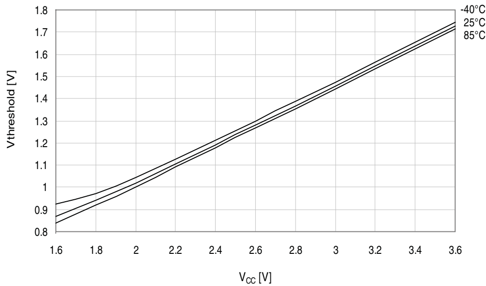
Figure 34-231. I/O pin input threshold voltage vs. V_{CC} . V_{IL} I/O pin read as “0”.
