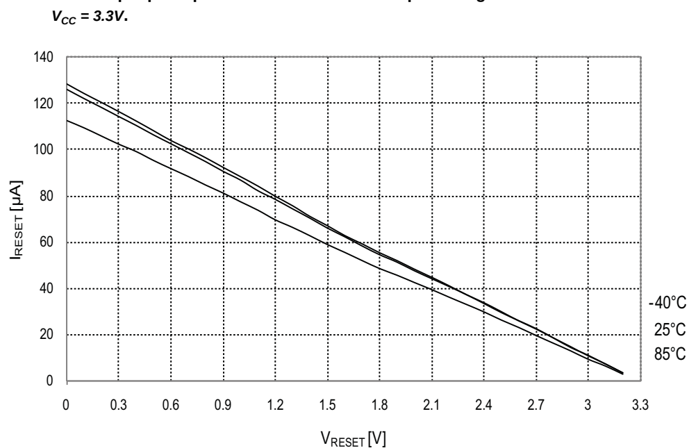
Figure 34-187. Reset pin pull-up resistor current vs. reset pin voltage.
