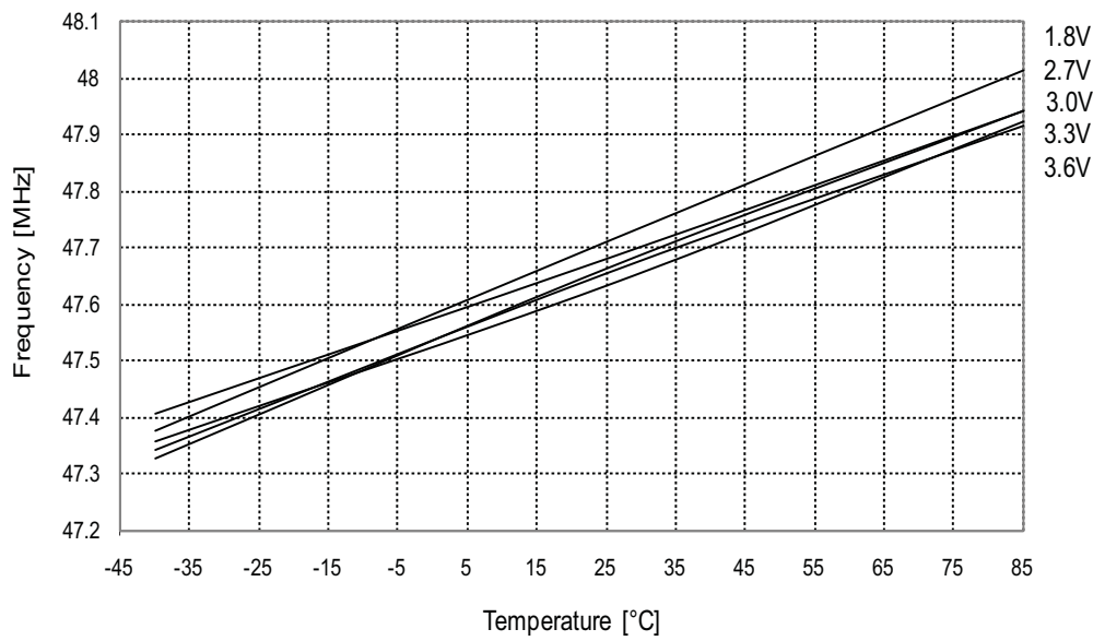
Figure 34-200. 48MHz internal oscillator frequency vs. temperature. DFLL enabled, from the 32.768kHz internal oscillator.
