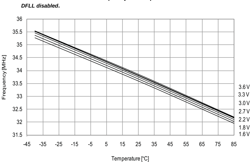
Figure 34-60. 32MHz internal oscillator frequency vs. temperature.
