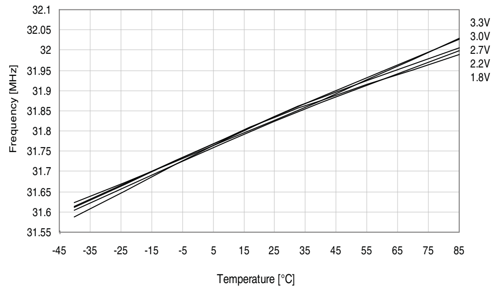
Figure 34-263. 32MHz internal oscillator frequency vs. temperature. DFLL enabled, from the 32.768kHz internal oscillator.
