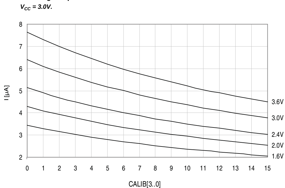
Figure 34-313. Analog comparator current source vs. calibration value.
