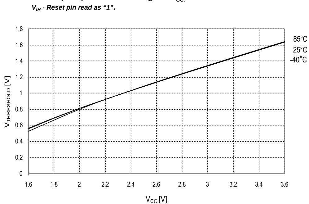
Figure 34-188. Reset pin input threshold voltage vs. V_{CC} .
