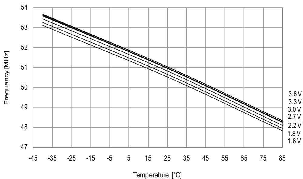
Figure 34-132. 48MHz internal oscillator frequency vs. temperature.
