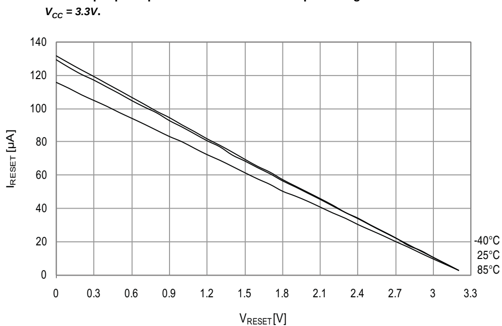
Figure 34-120. Reset pin pull-up resistor current vs. reset pin voltage.
