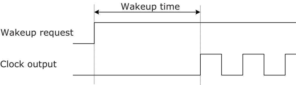
Figure 33-30.Wakeup time definition.
