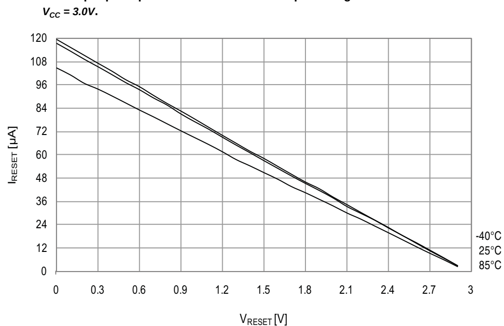
Figure 34-51. Reset pin pull-up resistor current vs. reset pin voltage.
