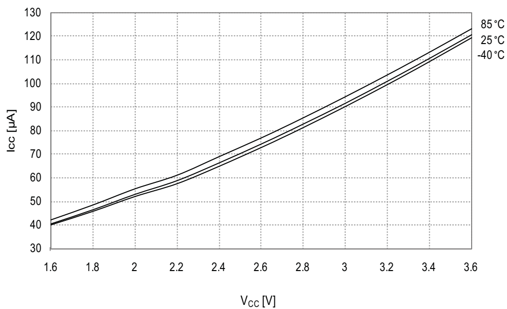
Figure 34-12. Idle mode supply current vs. V_{CC} .
