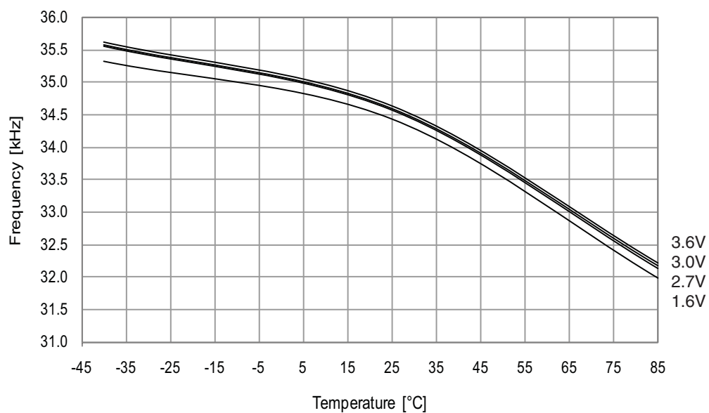
Figure 34-122. Ultra Low-Power internal oscillator frequency vs. temperature.
