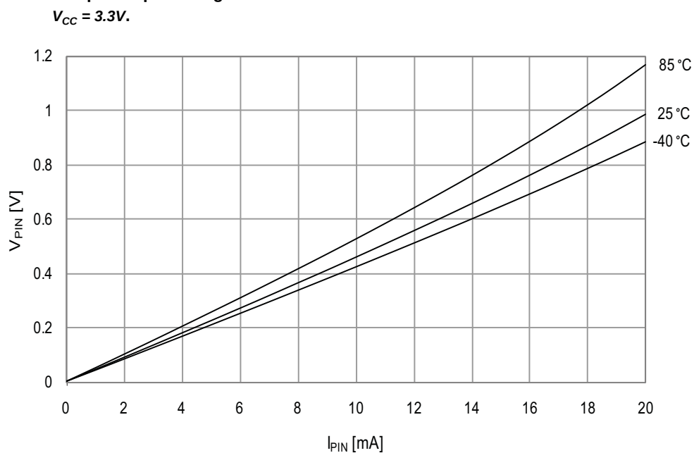
Figure 34-95. I/O pin output voltage vs. sink current.
