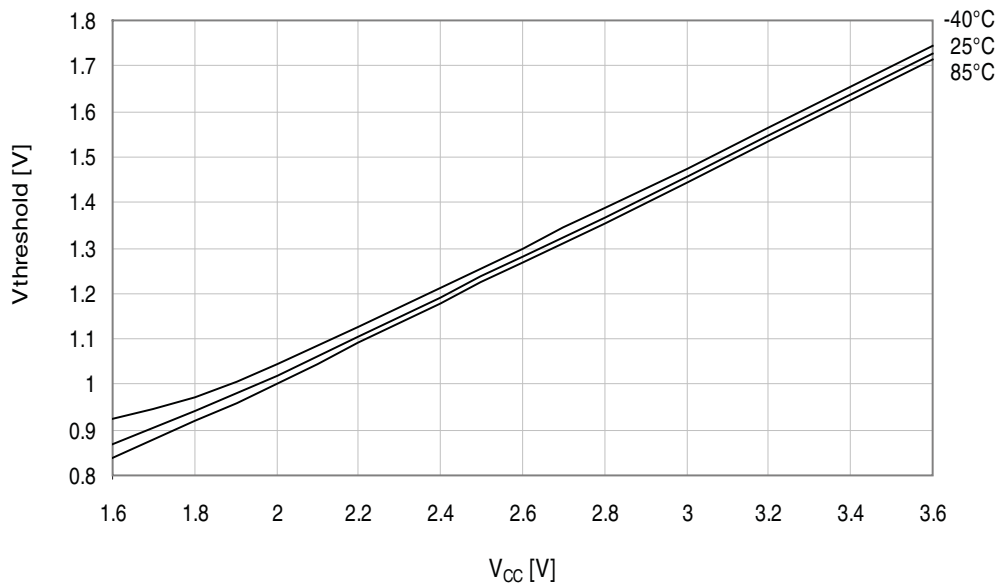
Figure 34-298. I/O pin input threshold voltage vs. V_{CC} . V_{IL} I/O pin read as "0".
