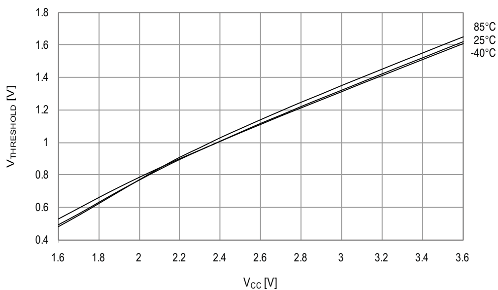
Figure 34-121. Reset pin input threshold voltage vs. V_{CC} .
