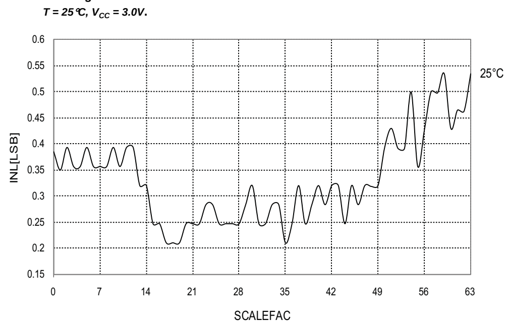
Figure 34-180. Voltage scaler INL vs. SCALEFAC.
