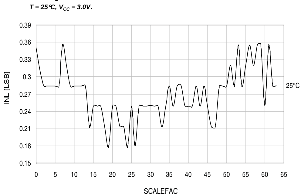
Figure 34-314. Voltage scaler INL vs. SCALEFAC.
