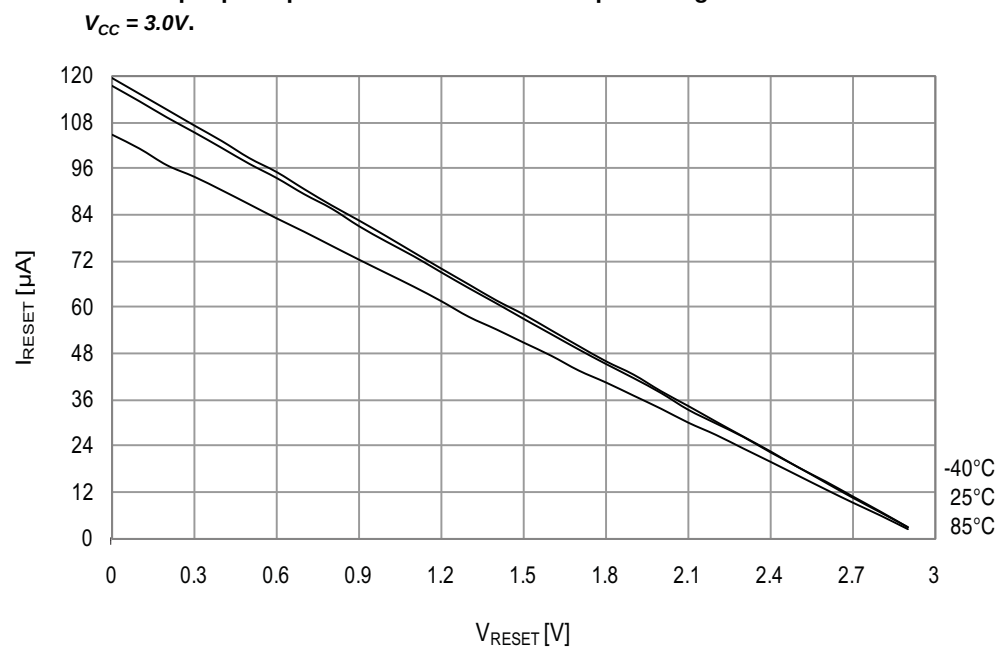
Figure 34-119. Reset pin pull-up resistor current vs. reset pin voltage.
