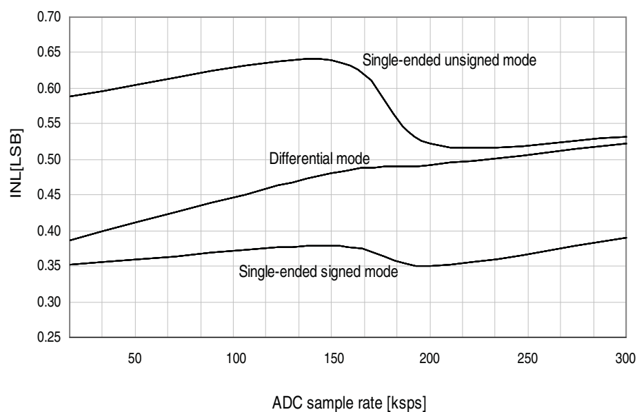
Figure 34-167. INL error vs. sample rate. T = 25^{\circ}\text{C} , V_{CC} = 3.6\text{V} , V_{REF} = 3.0\text{V external} .
