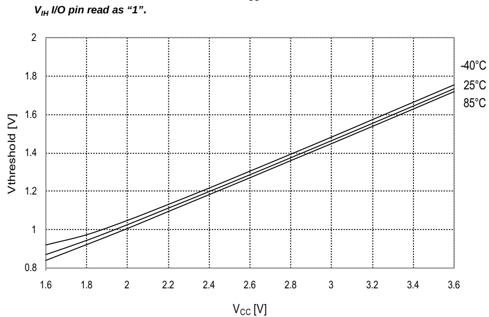
Figure 34-163. I/O pin input threshold voltage vs. V_{CC} .
