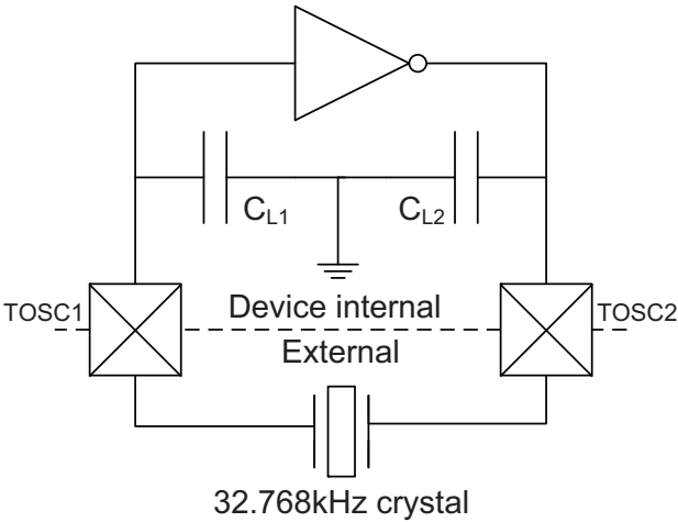
Figure 33-18.TOSC input capacitance.
