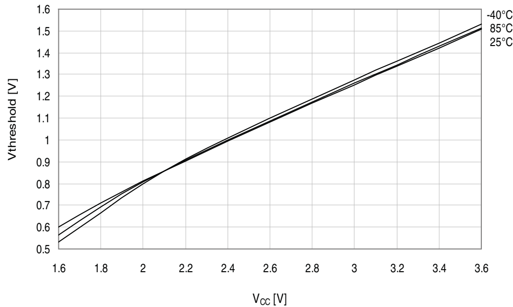
Figure 34-231. I/O pin input threshold voltage vs. V_{CC} . V_{IL} I/O pin read as “0”.
