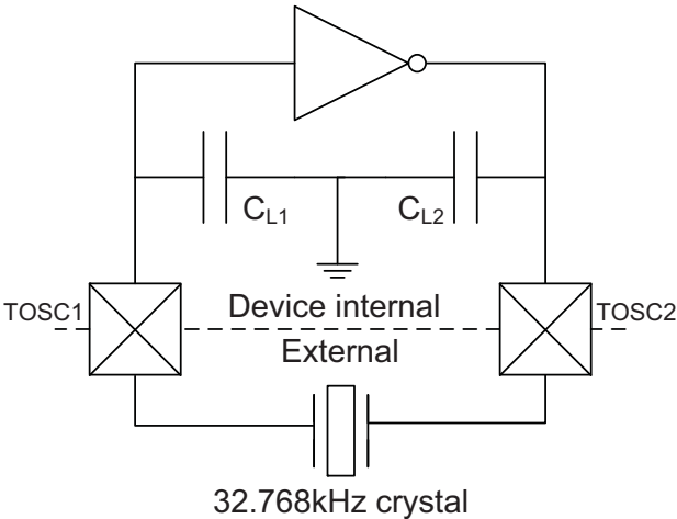
Figure 33-32.TOSC input capacitance.
