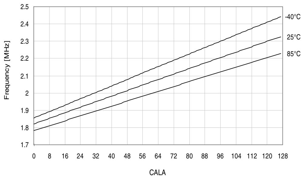
Figure 34-261. 2MHz internal oscillator frequency vs. CALA calibration value. V_{CC} = 3V .
