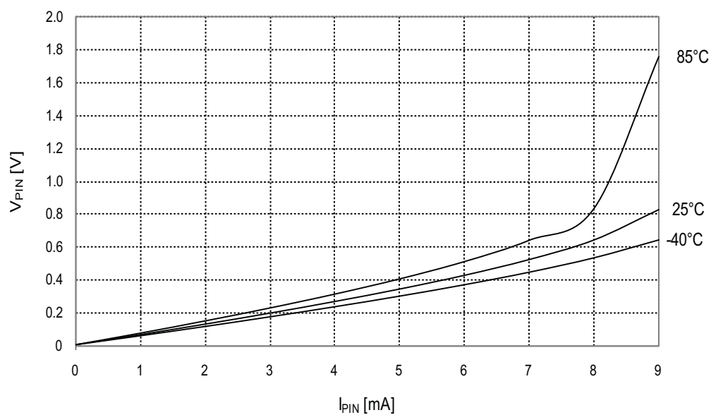
Figure 34-160. I/O pin output voltage vs. sink current.
