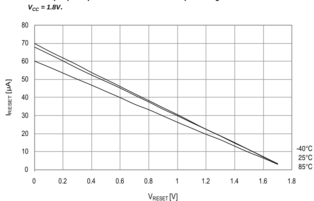
Figure 34-50. Reset pin pull-up resistor current vs. reset pin voltage.
