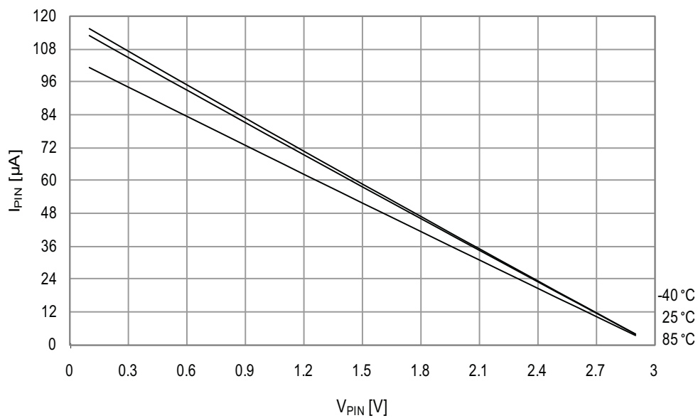
Figure 34-88. I/O pin pull-up resistor current vs. input voltage. V_{CC} = 3.0V .
