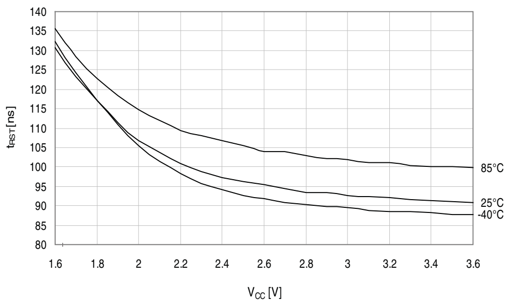
Figure 34-251. Minimum Reset pin pulse width vs. V_{CC} .
