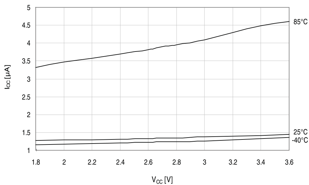
Figure 34-219. Power-down mode supply current vs. V_{CC} .
