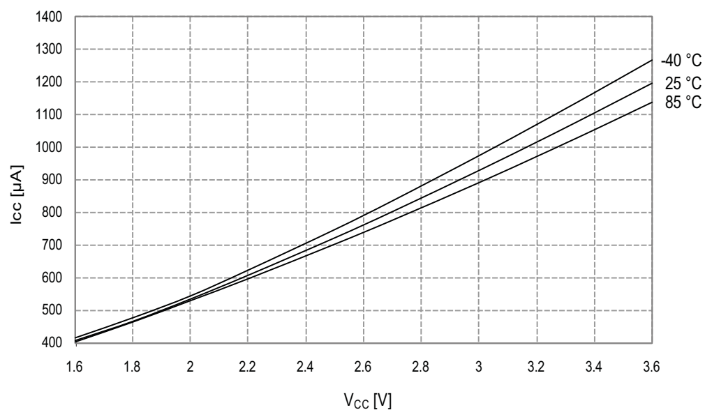
Figure 34-74. Active mode supply current vs. V_{CC} .
