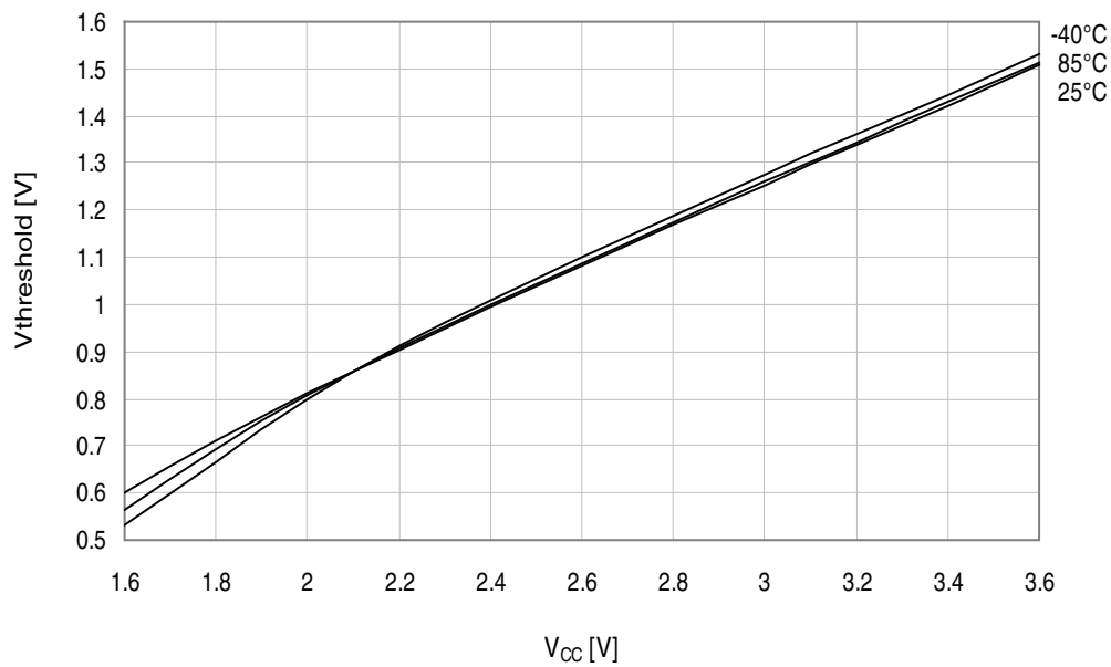
Figure 34-298. I/O pin input threshold voltage vs. V_{CC} . V_{IL} I/O pin read as "0".
