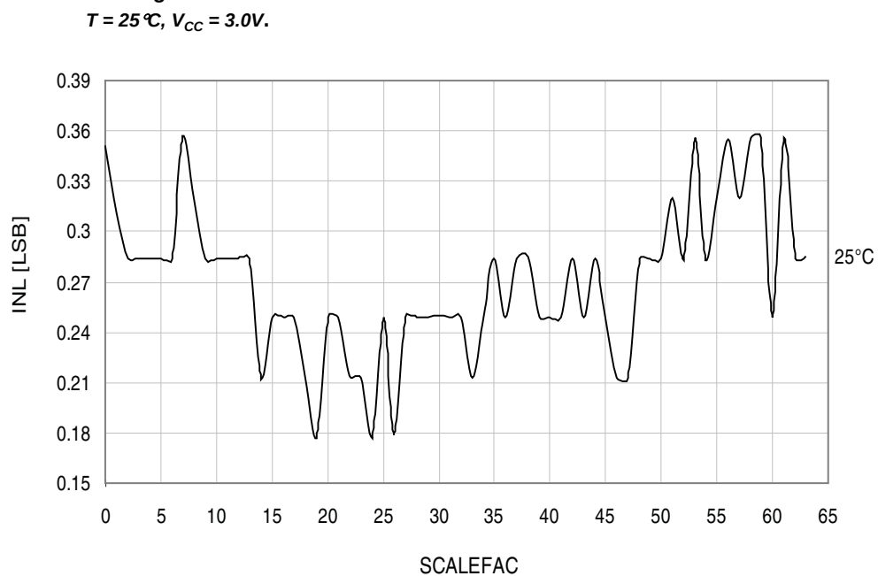
Figure 34-247. Voltage scaler INL vs. SCALEFAC.
