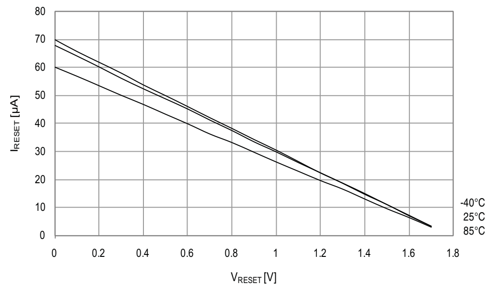
Figure 34-118. Reset pin pull-up resistor current vs. reset pin voltage. V_{CC} = 1.8V .
