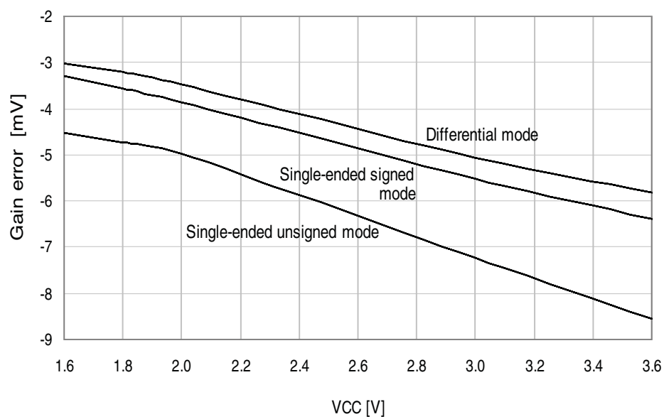
Figure 34-106. Gain error vs. V_{CC} .
