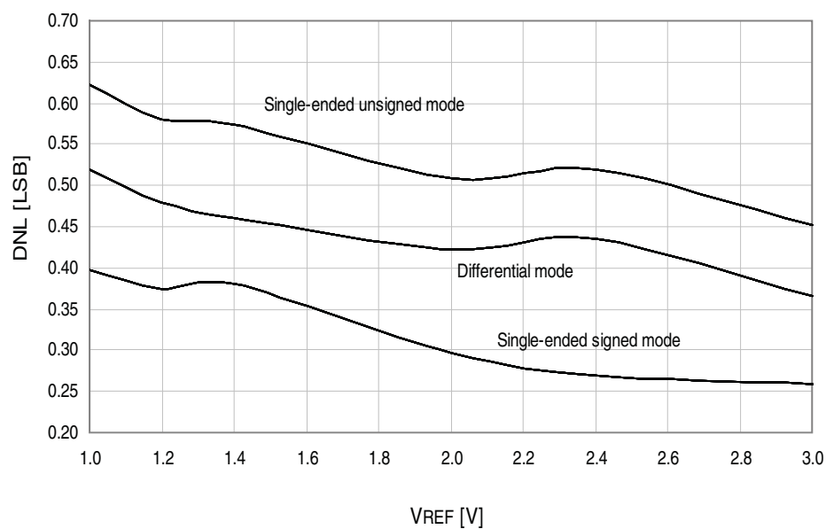
Figure 34-169. DNL error vs. external V_{REF} . T = 25^{\circ}\text{C} , V_{CC} = 3.6\text{V} , external reference.
