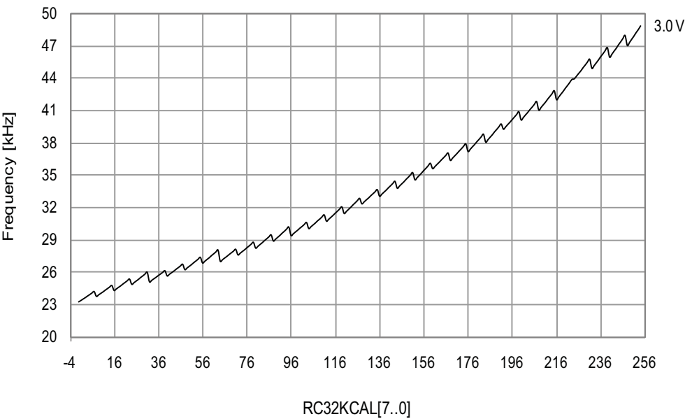
Figure 34-124. 32.768kHz internal oscillator frequency vs. calibration value. V_{CC} = 3.0V , T = 25^{\circ}C .
