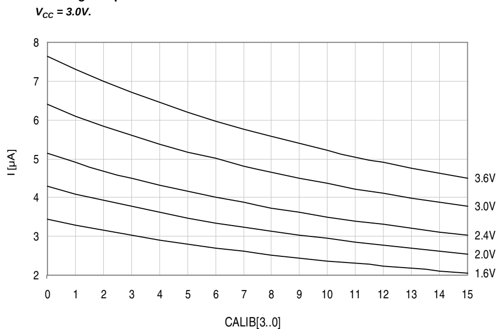
Figure 34-246. Analog comparator current source vs. calibration value.
