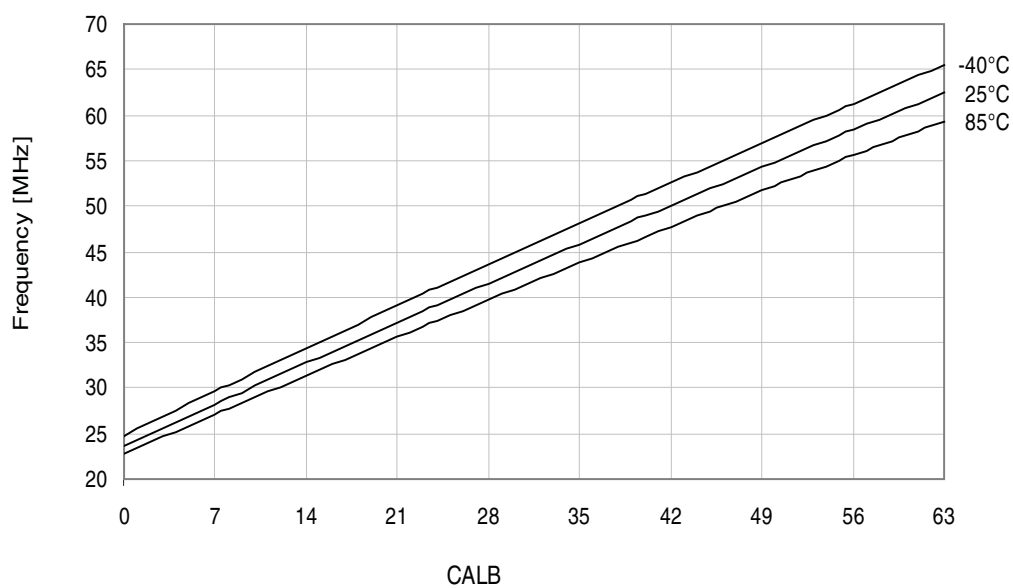
Figure 34-265. 32MHz internal oscillator frequency vs. CALB calibration value.
