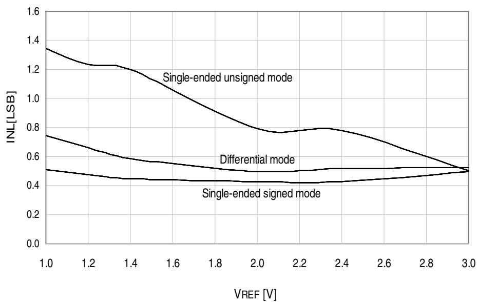
Figure 34-300. INL error vs. external V_{REF} .
