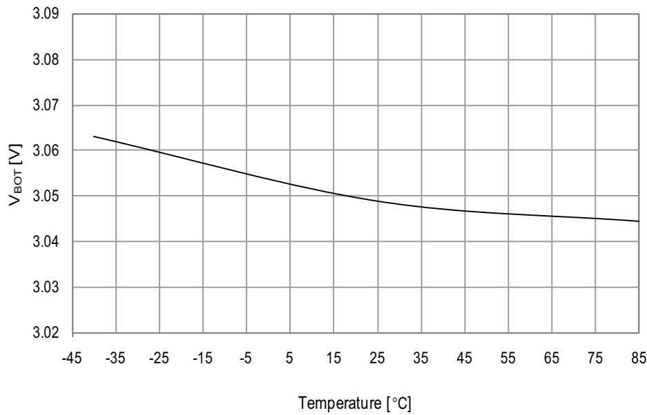
Figure 34-116. BOD thresholds vs. temperature. BOD level = 3.0V.
