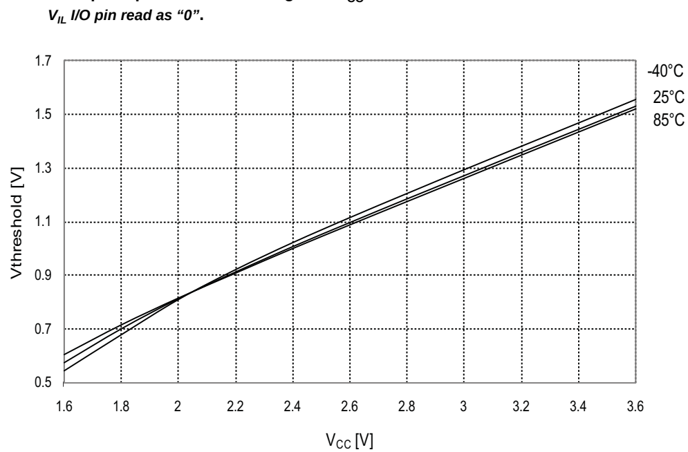
Figure 34-164. I/O pin input threshold voltage vs. V_{CC} .
