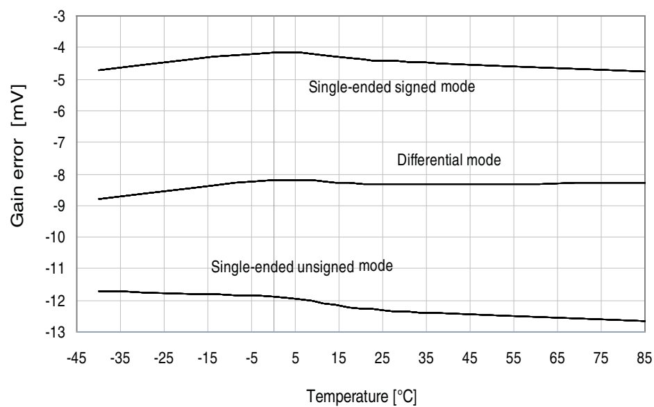
Figure 34-108. Gain error vs. temperature.
