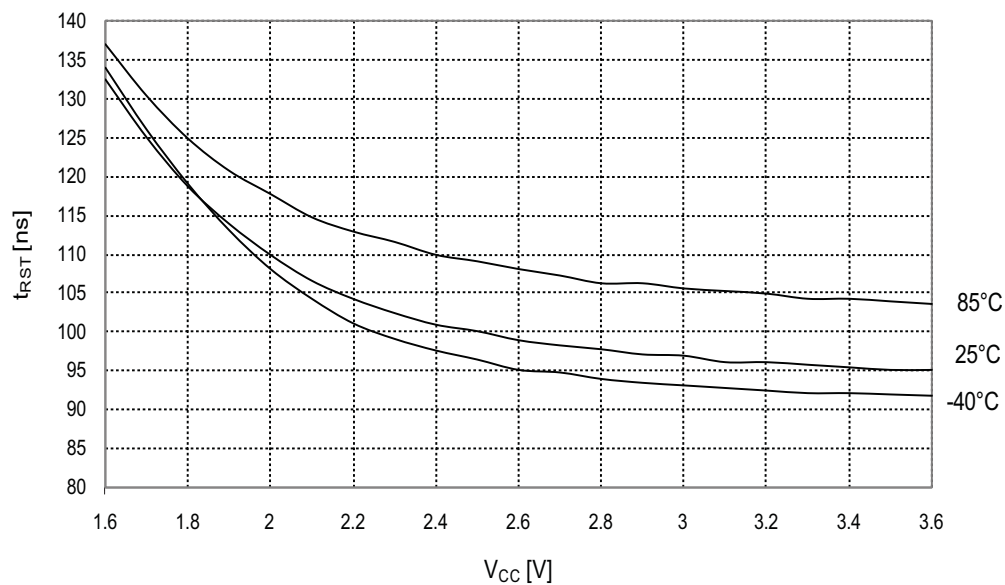
Figure 34-184. Minimum Reset pin pulse width vs. V_{CC} .
