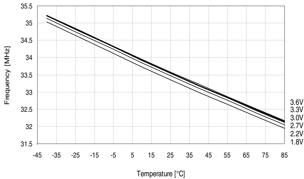
Figure 34-330. 32MHz internal oscillator frequency vs. temperature. DFLL enabled, from the 32.768kHz internal oscillator.
