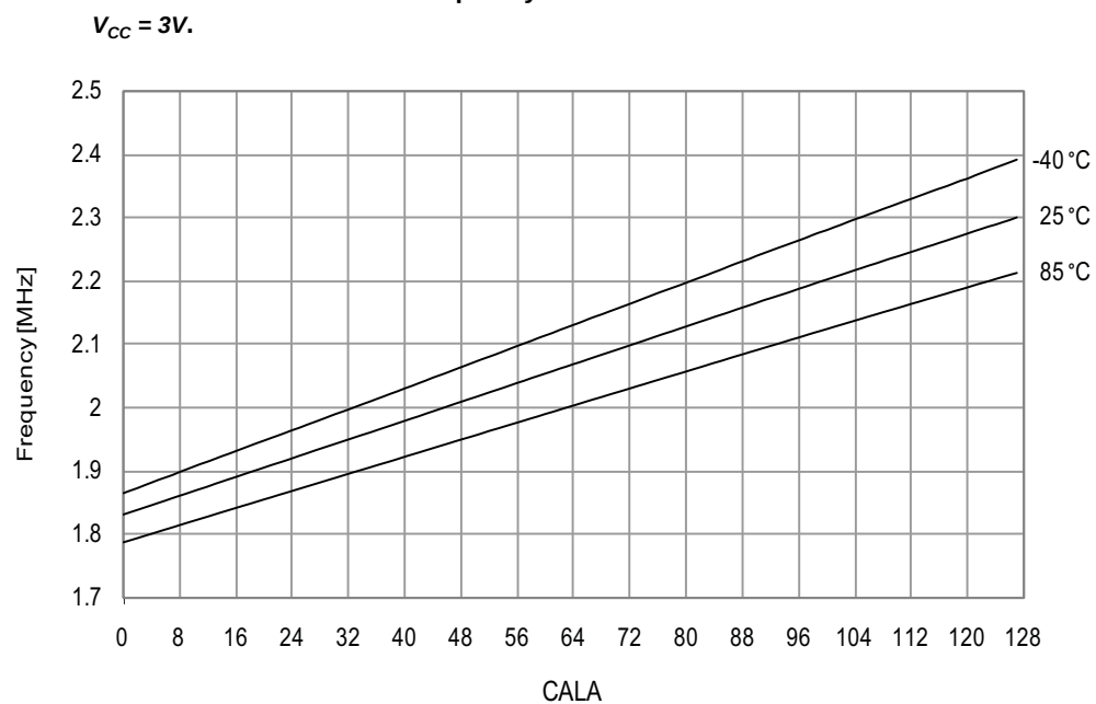
Figure 34-59. 2MHz internal oscillator frequency vs. CALA calibration value.
