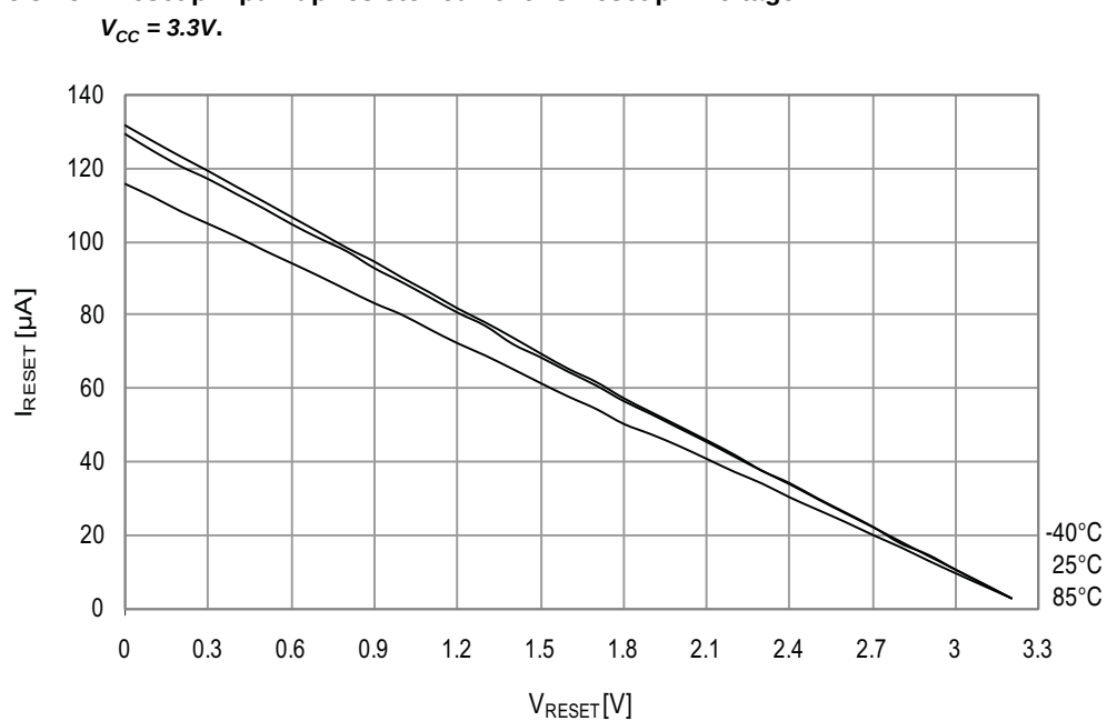
Figure 34-52. Reset pin pull-up resistor current vs. reset pin voltage.
