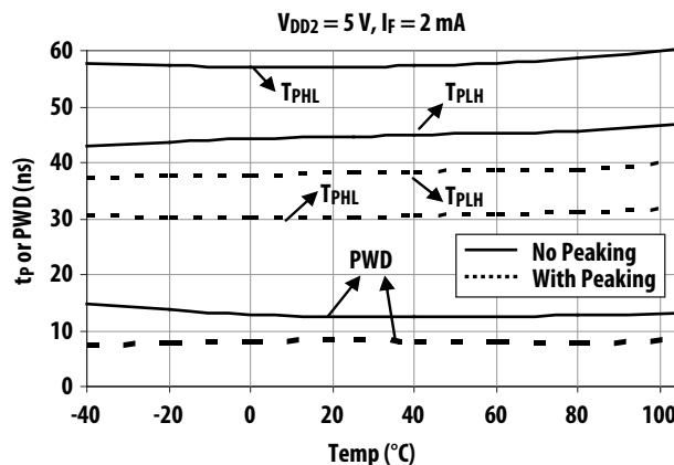
(i) V_{DD} = 5V , C_{peak} = 47pF , R_1 = 845\Omega
