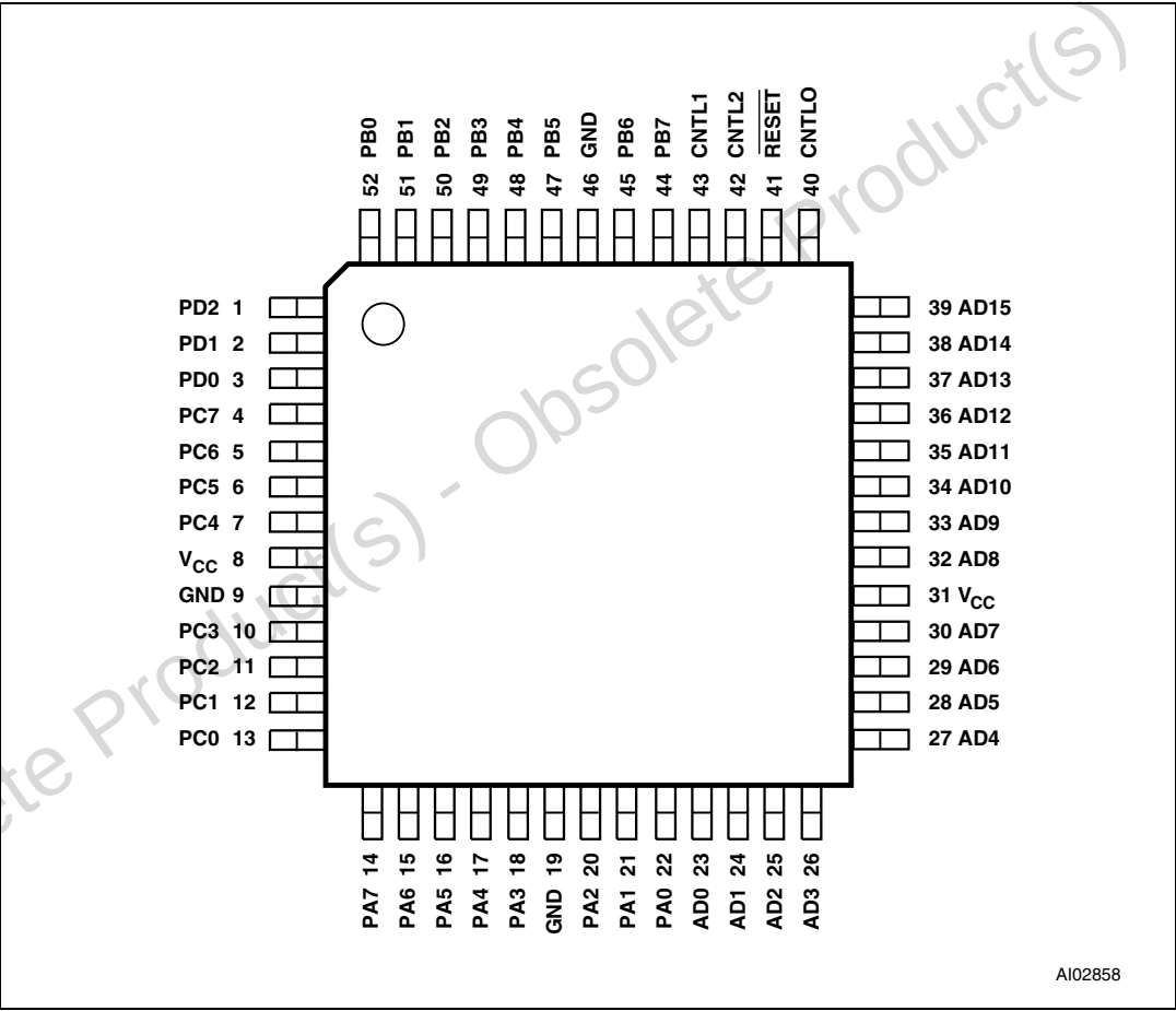
Figure 1. PQFP52 connections
