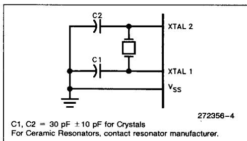
Figure 3. Oscillator Connections
