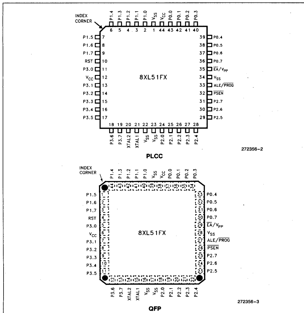
Figure 2. Pin Connections
