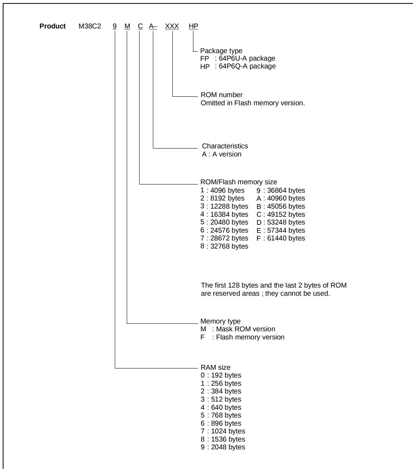
Fig. 3 Part numbering
