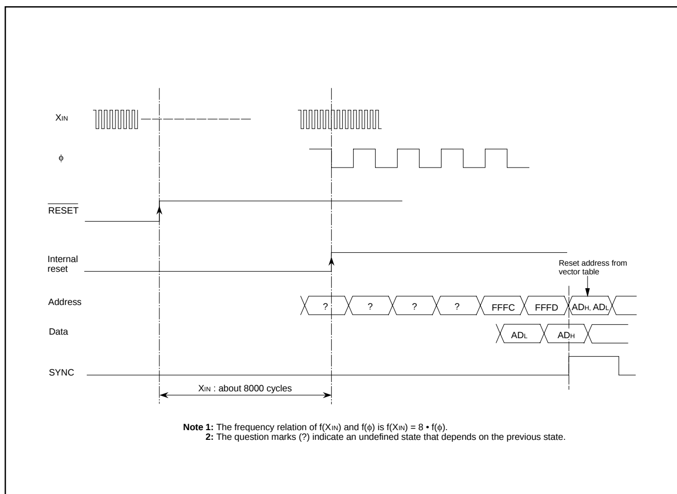
Fig. 48 Reset sequence
