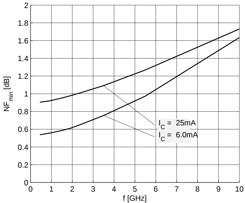
Figure 5-18 Noise Figure NF_{min} = f(f) , V_{CE} = 3\text{ V} , I_C = 6 / 25\text{ mA} , Z_S = Z_{opt}
