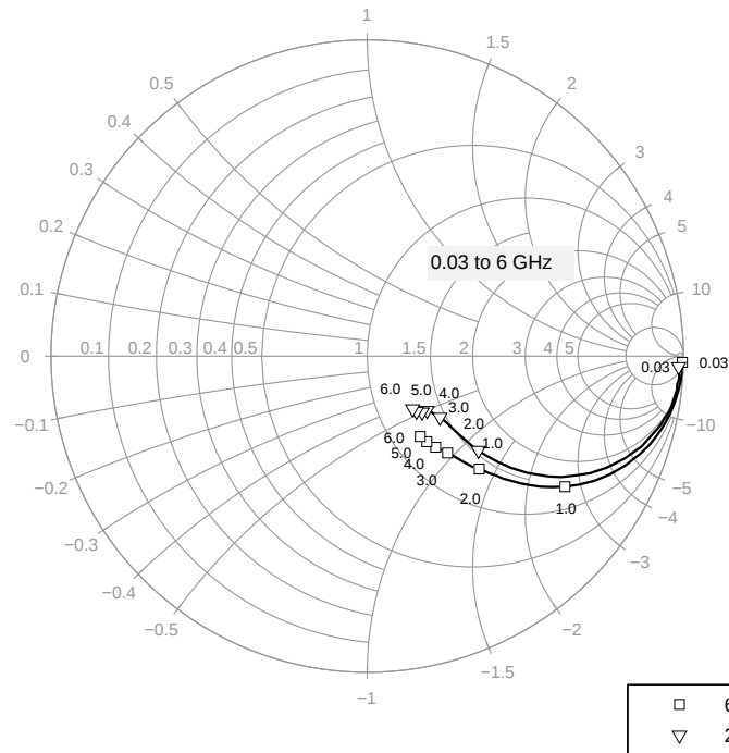
Figure 5-17 Output Matching S_{22} = f(f) , V_{CE} = 3\text{ V} , I_C = 6 / 25\text{ mA}
