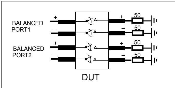
Fig 1. Crosstalk Setup
