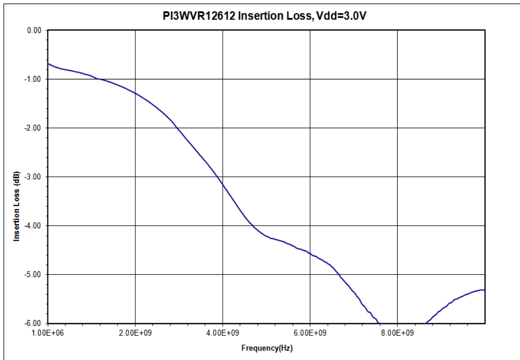
Fig 6. Insertion Loss
