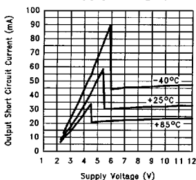
Output Short Circuit Current vs Supply Voltage (Sourcing)
