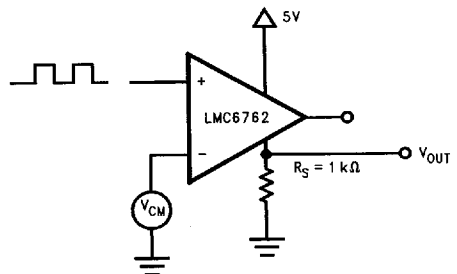
FIGURE 3. LMC6762 Circuit for Measurement of the Shoot-Through Current
