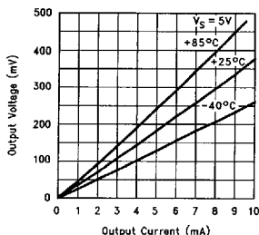
Output Voltage vs Output Current (Sinking)
