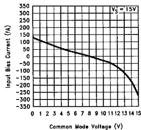
Input Current vs Common-Mode Voltage
