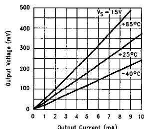
Output Voltage vs Output Current (Sinking)
