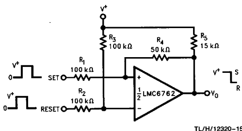
FIGURE 7. Bi-Stable Multivibrator
