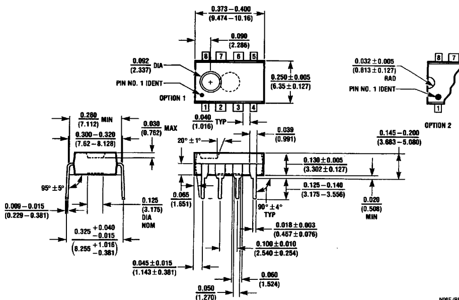
8-Pin Molded Dual-In-Line Package Order Number LMC6762AI or LMC6762BI NS Package Number N08E
