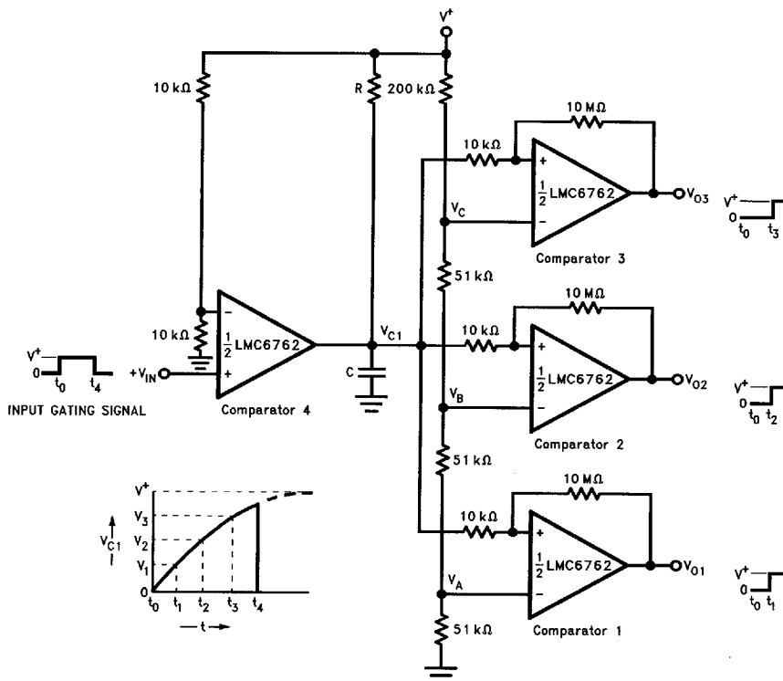
FIGURE 10. Time Delay Generator
