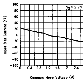
Input Current vs Common-Mode Voltage
