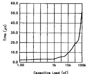
Response Time vs Capacitive Load
