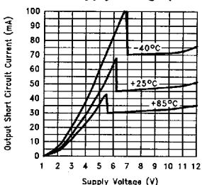
Output Short Circuit Current vs Supply Voltage (Sinking)
