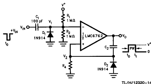
FIGURE 6. One-Shot Multivibrator
