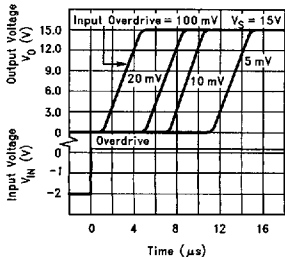
Response Time for Overdrive ( t_{PLH} )
