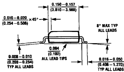
8-Pin Small Outline Package Order Number LMC6762AI or LMC6762BI NS Package Number M08A
