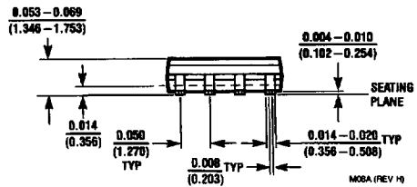
8-Pin Small Outline Package Order Number LMC6762AI or LMC6762BI NS Package Number M08A
