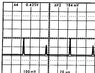
FIGURE 4. Measurement of the Shoot-Through Current
