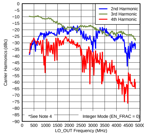
Figure 60. LO Harmonics
