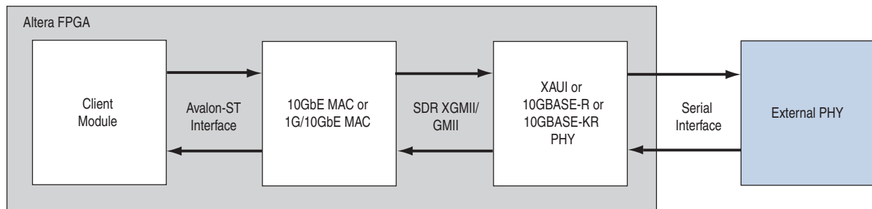
Figure 1–1. Typical Application of 10GbE MAC
