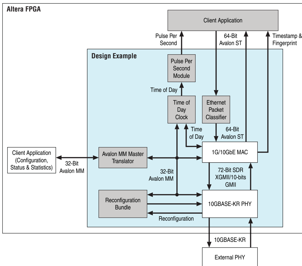
Figure 6–1. 1G/10GbE MAC with IEEE 1588v2 Design Example Block Diagram
