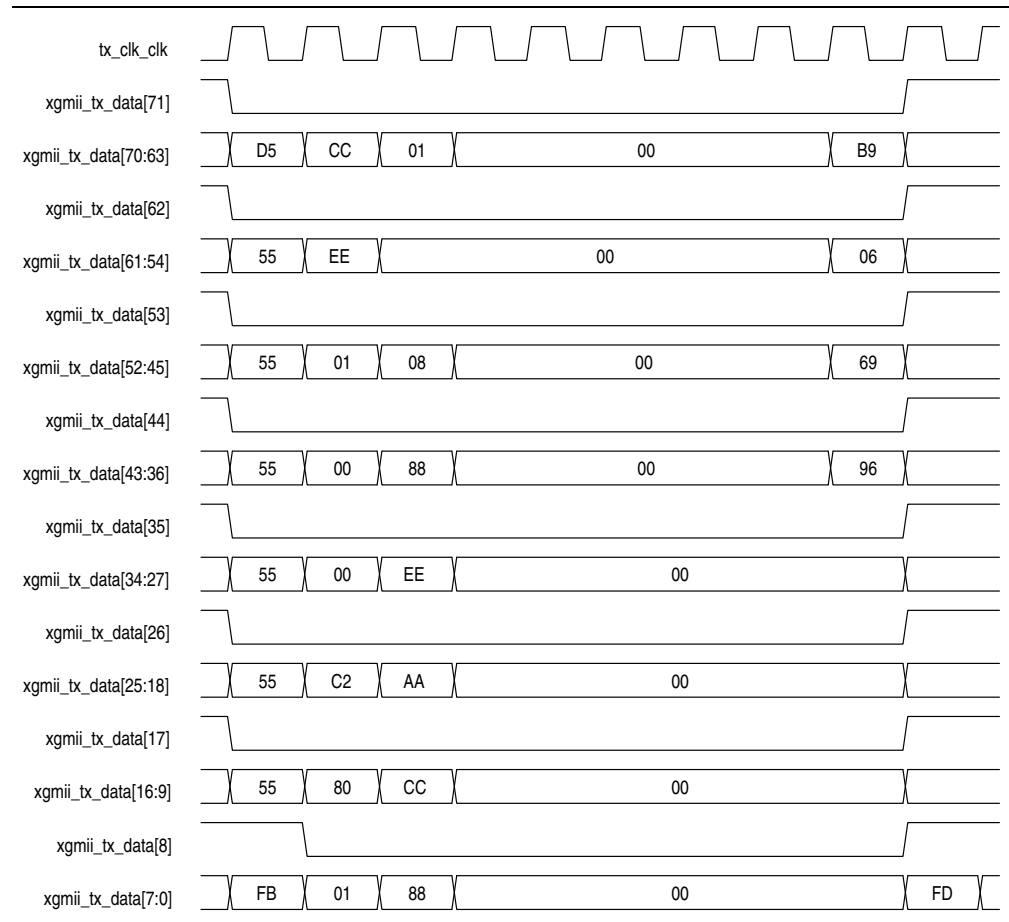
Figure 7–9. XON Pause Frame Transmission
