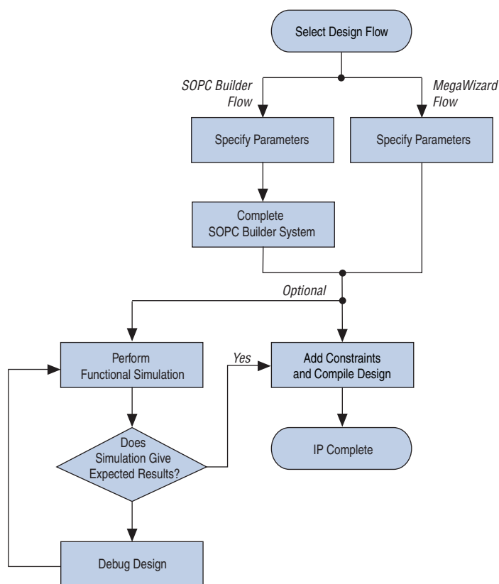
Figure 2-2. Design Flows
