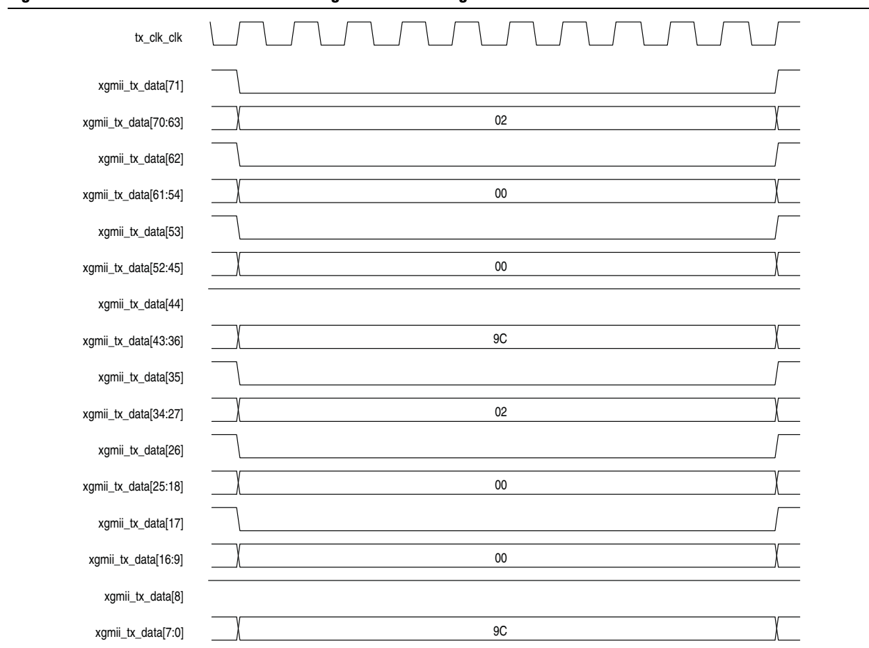
Figure 7-11. XGMII TX interface Transmitting Remote Fault Signal
