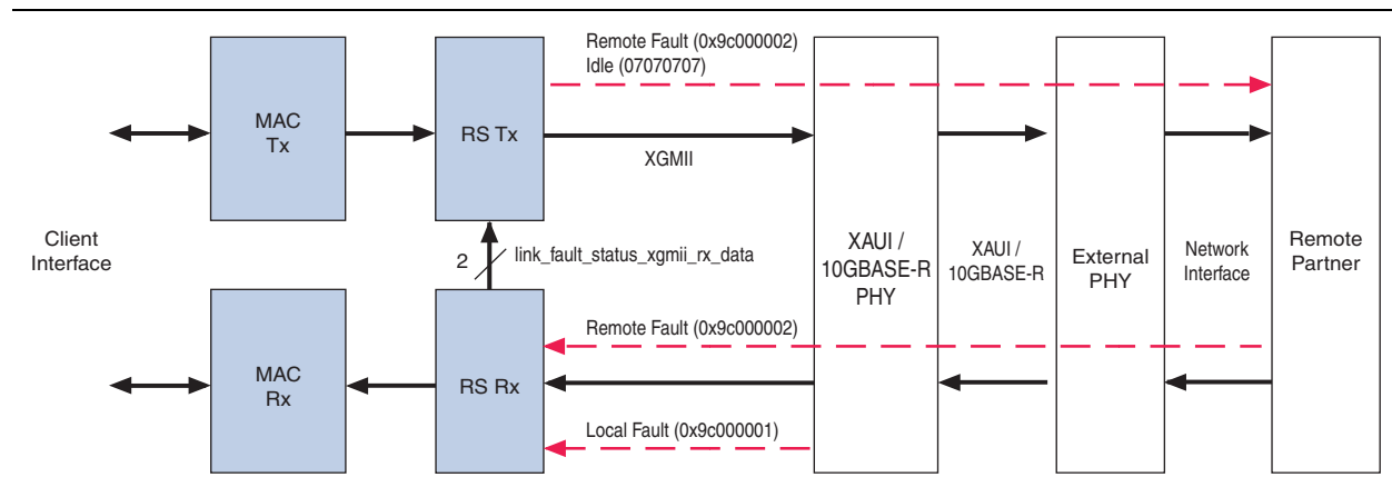
Figure 7–10. Fault Signaling
