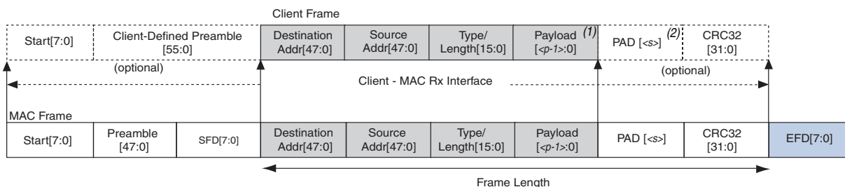
Figure 7-7. Typical Client Frame at Receive Interface
