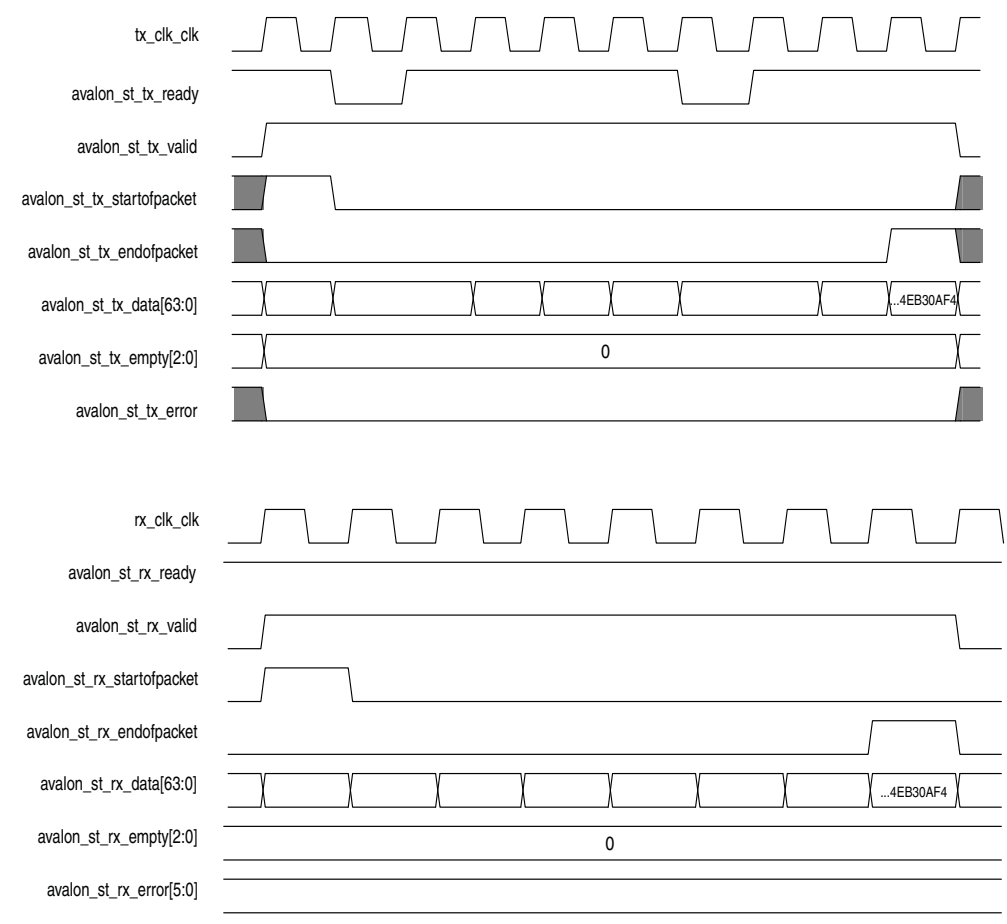
Figure 7–5. Avalon-ST Transmit and Receive Interface with CRC-32 Computation Disabled
