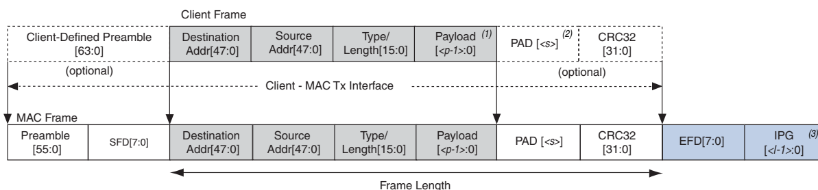
Figure 7-3. Typical Client Frame at Transmit Interface
