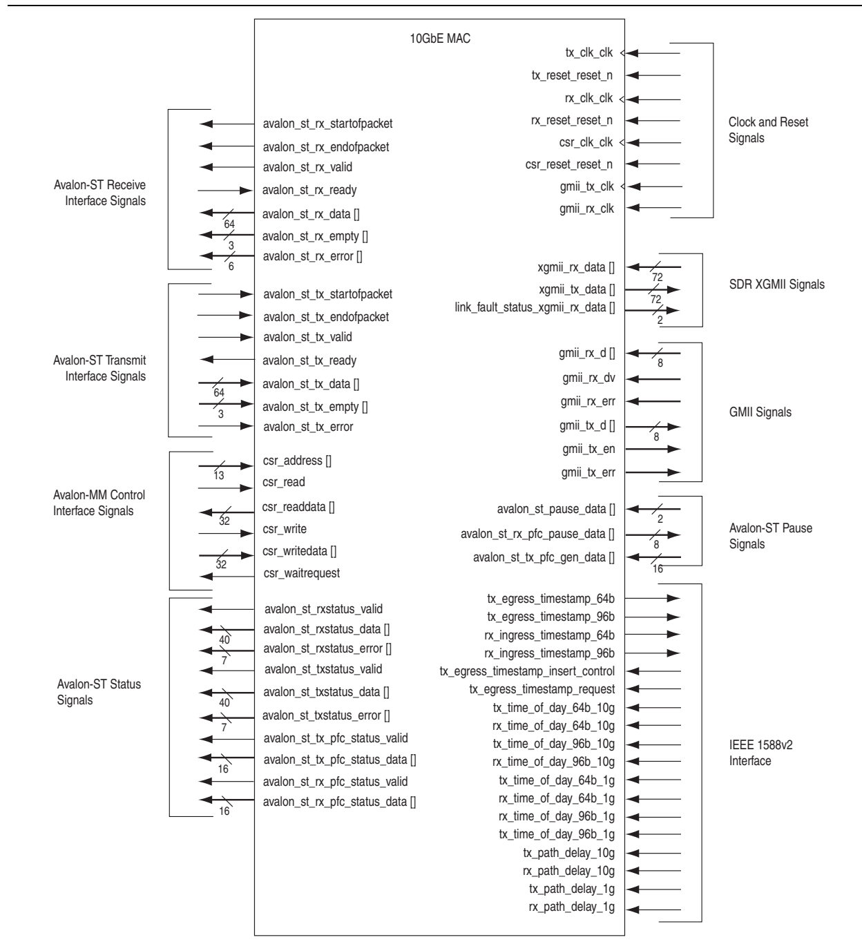
Figure 9–1. 10GbE MAC
