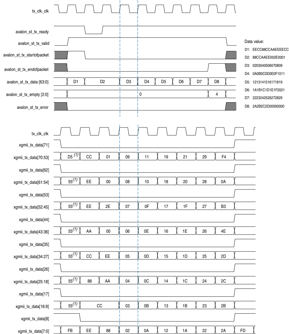
Figure 7-6. Endian Conversion
