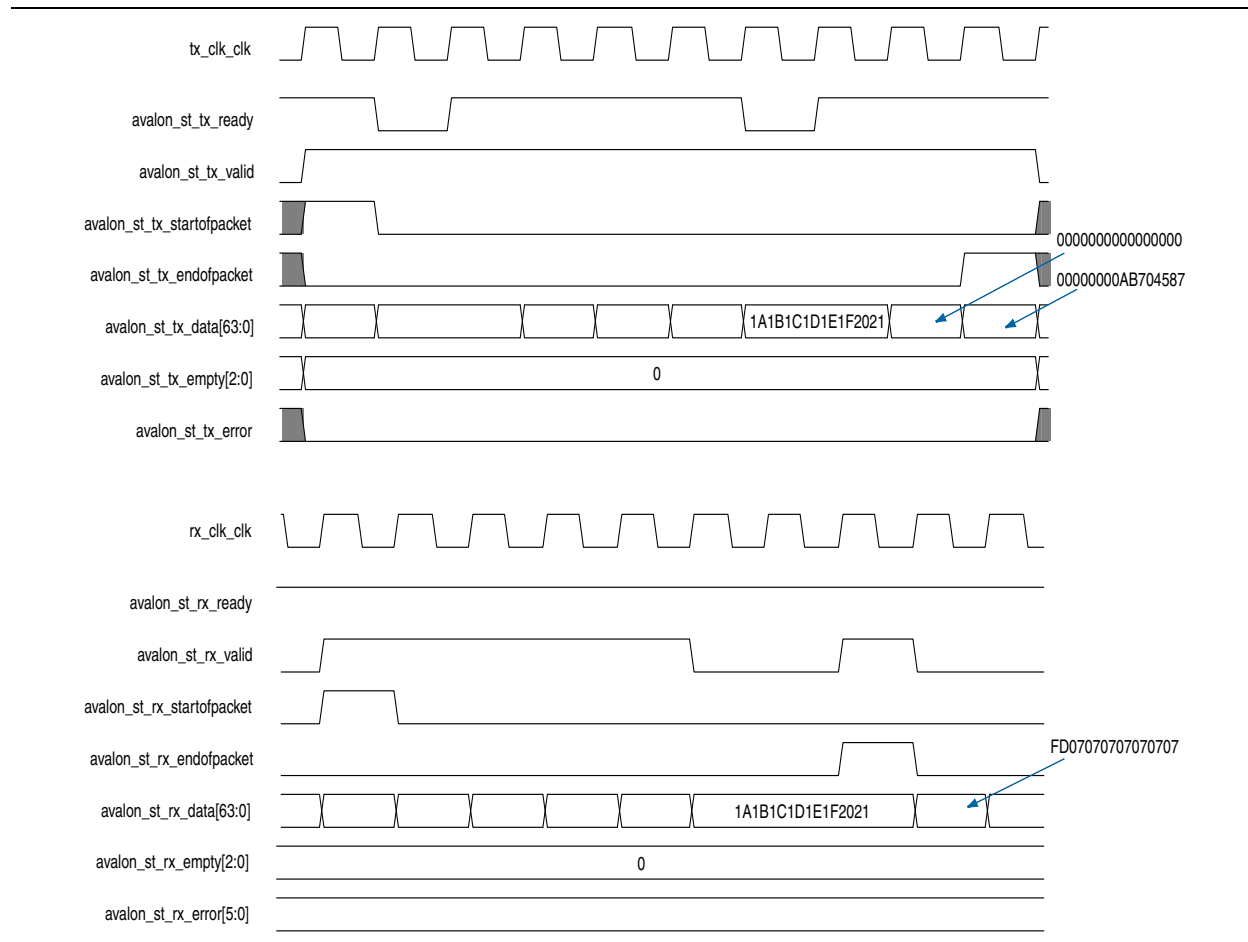
Figure 7-8. Avalon-ST Transmit and Receive Interface with Pad Bytes and CRC-32 Field Removed
