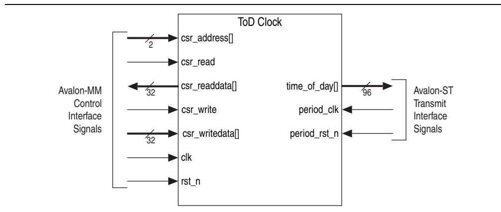
Figure B-1. ToD Clock Interface Signals
