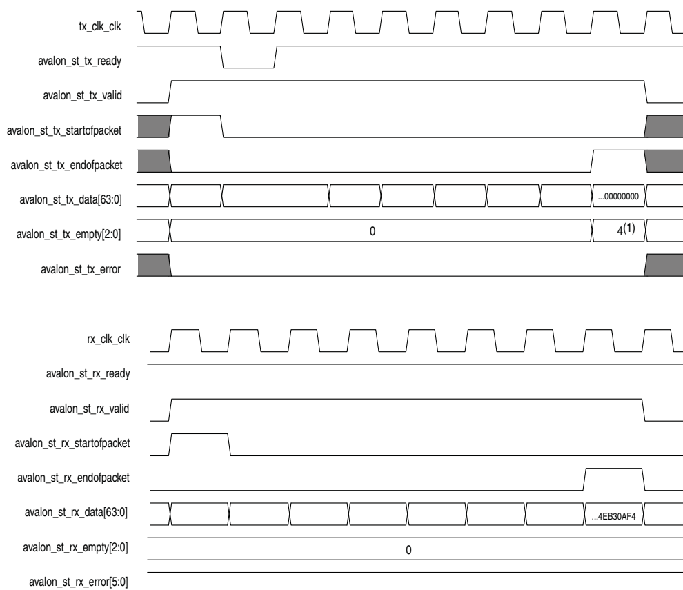
Figure 7-4. Avalon-ST Transmit and Receive Interface with CRC-32 Checksum Insertion
