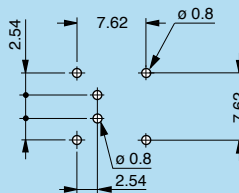
P19 - EPG-EXG (0B/1B.302) Solder mount
