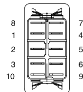
BOTTOM VIEW TERMINAL ARRANGEMENT 10 TERMINAL BASE
