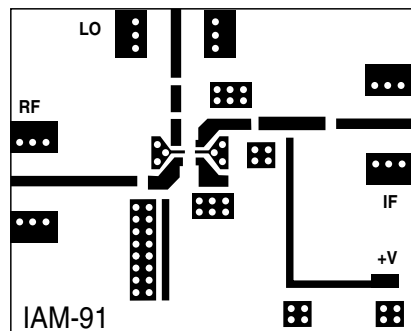
Figure 28. PCB Layout.
