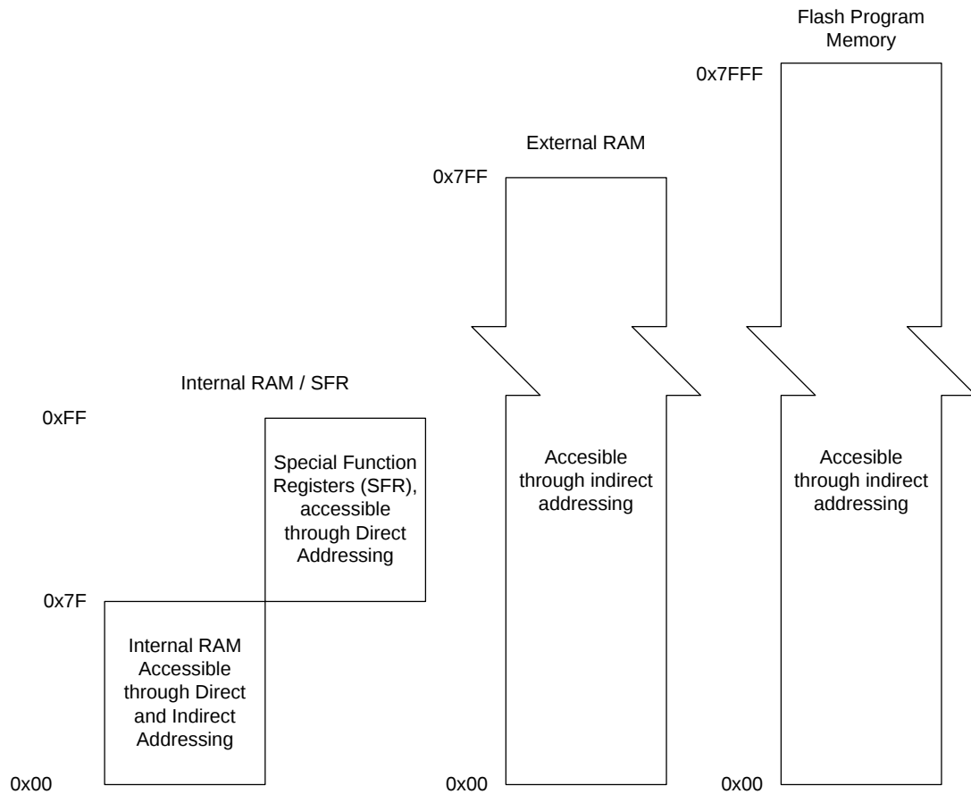
Figure 3. Memory Map
