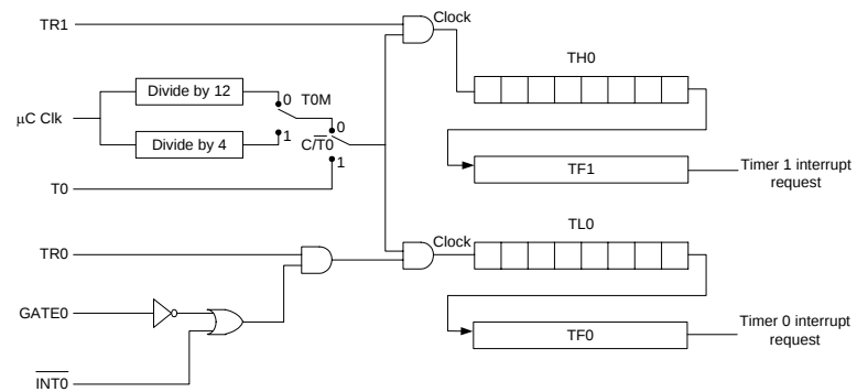
Figure 10. Mode 3 operation for Timer / Counter 0
