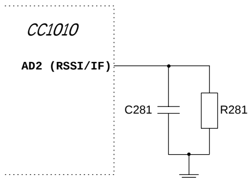
Figure 41. RSSI circuit
