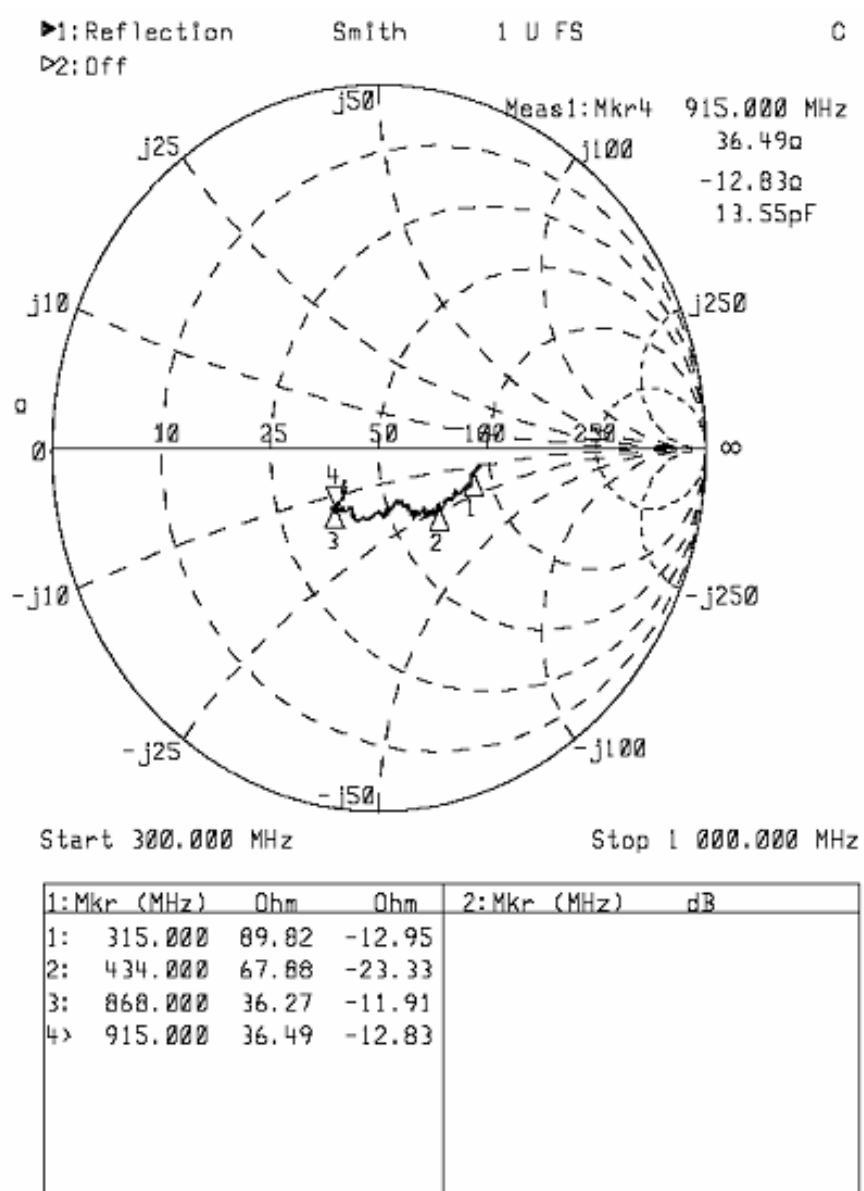
Figure 37. Typical LNA input impedance, 300 – 1000 MHz
