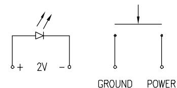
INTERNAL CIRCUIT
