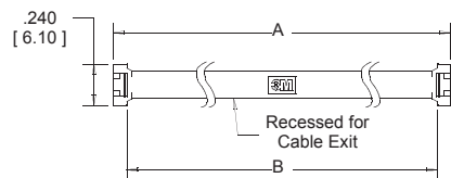
Top View of Cover
