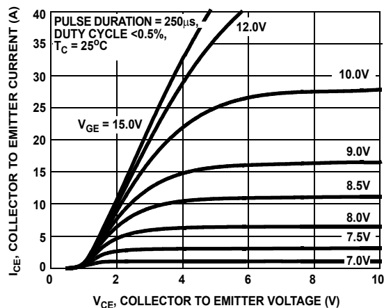
Figure 2. SATURATION CHARACTERISTICS
