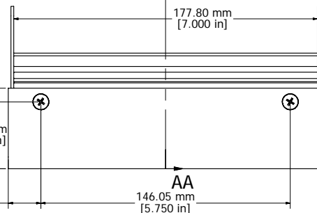
ASSEMBLY - VIEW FROM SIDE (OPEN)
