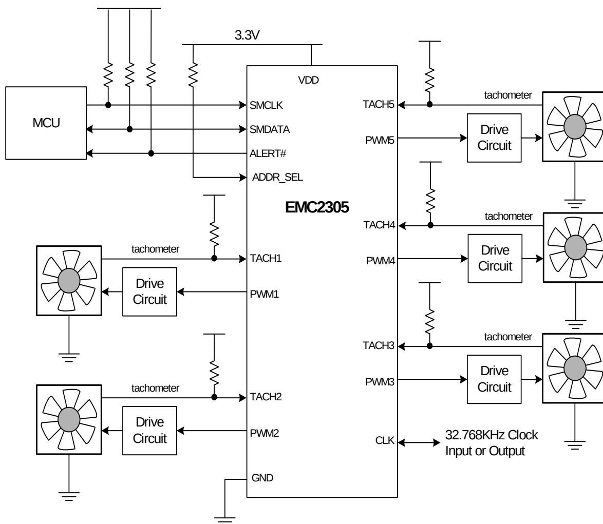
Figure 4.1 System Diagram of EMC2305
