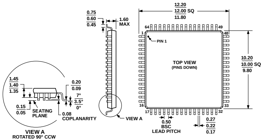
Figure 99. 64-Lead Low Profile Quad Flat Package [LQFP] (ST-64-2) Dimensions shown in millimeters
