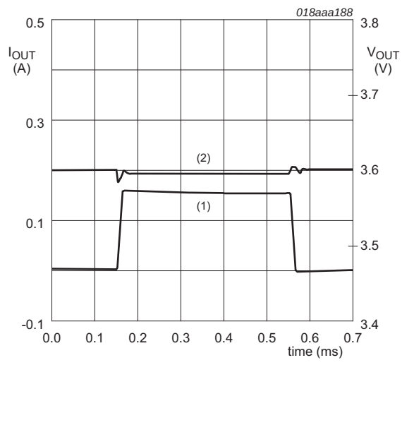
Fig 17. Load regulation for LD6816CX4/25P and LD6816CX4/C25P
