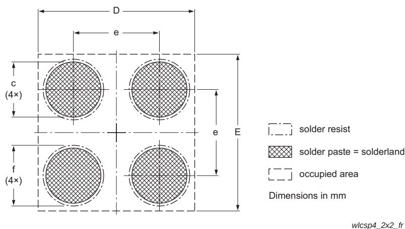
Fig 26. Reflow soldering footprint WLCSP4
