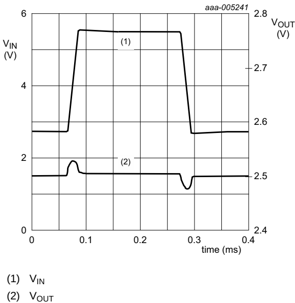
Fig 14. Line regulation for LD6816CX4/25P and LD6816CX4/C25P
