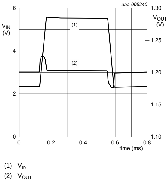
Fig 13. Line regulation for LD6816CX4/12H
