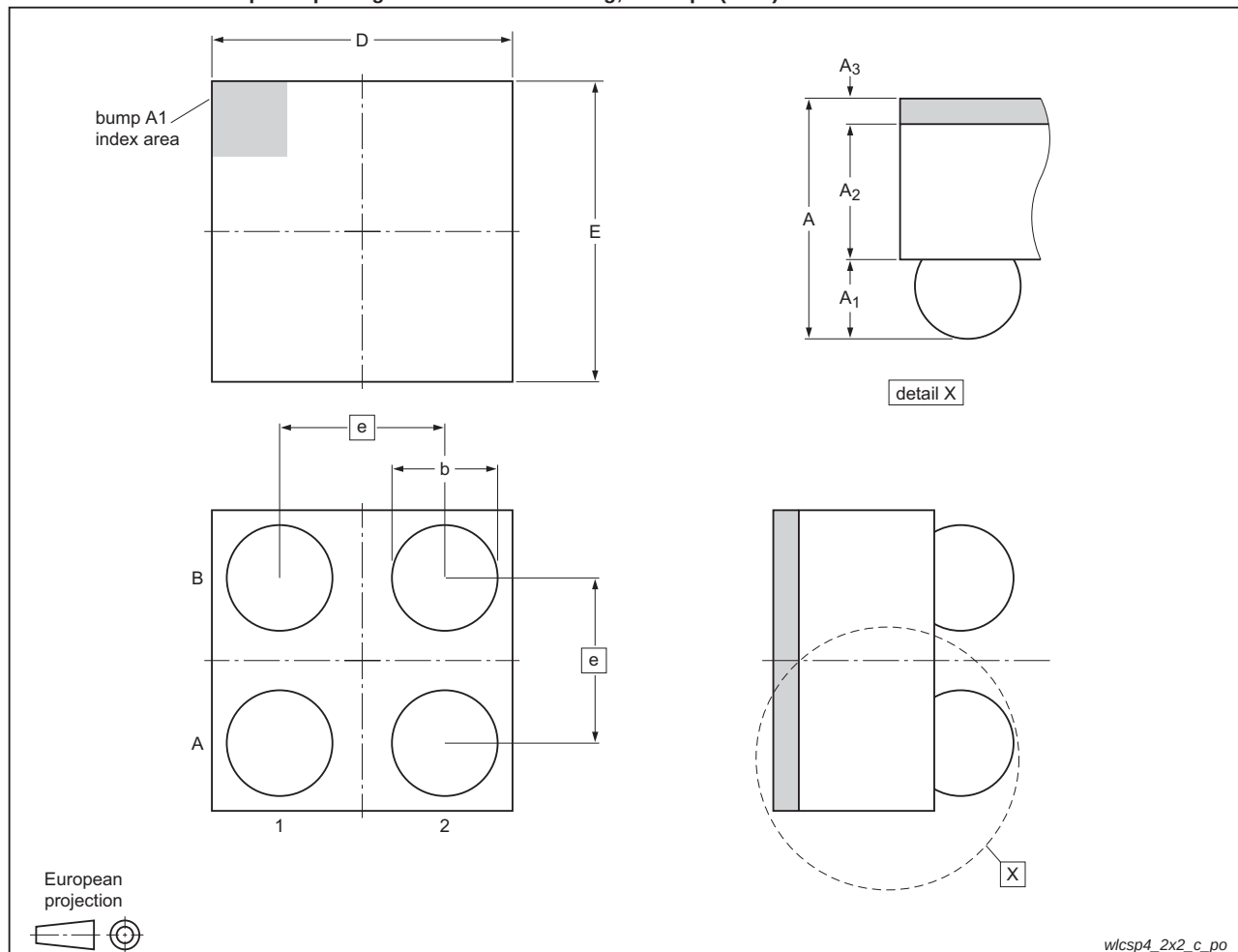
Fig 25. Package outline WLCSP4 with backside coating
