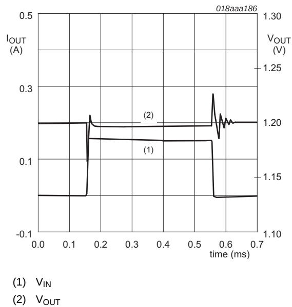
Fig 16. Load regulation for LD6816CX4/12H
