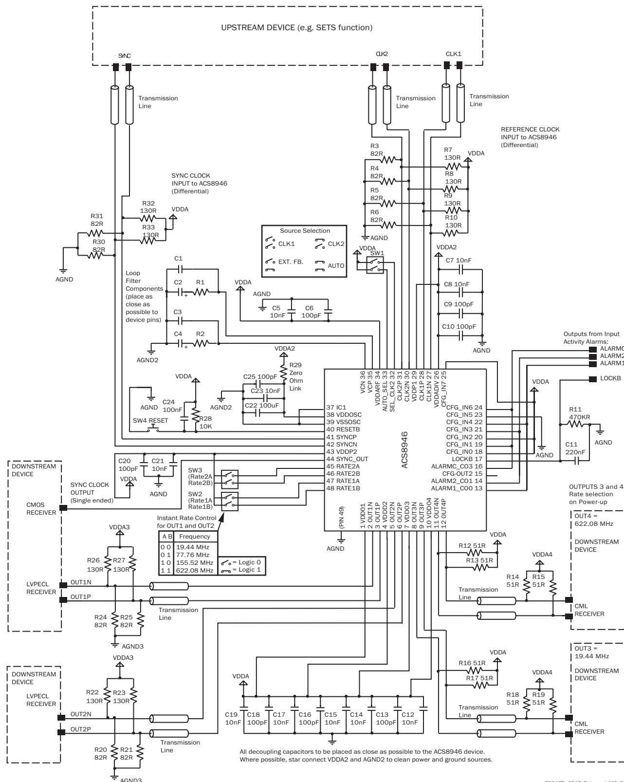
Figure 13 Generic Line Card Clock Source with Protection - Example Schematic
