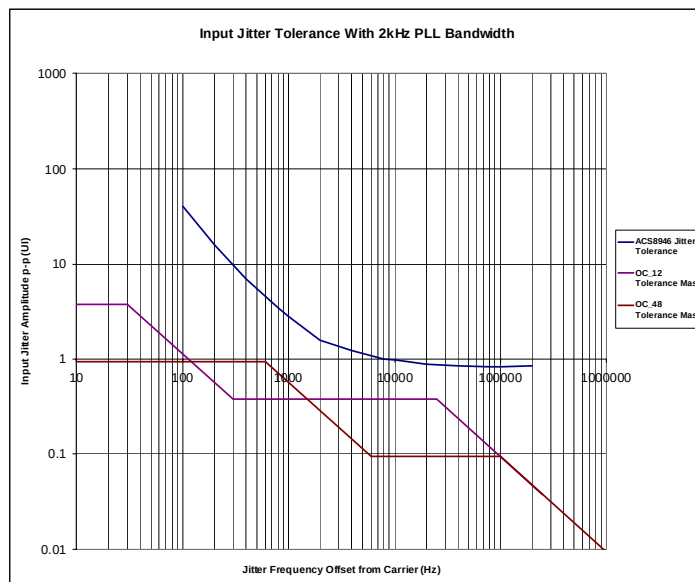
Figure 4 Jitter Tolerance ACS8946
