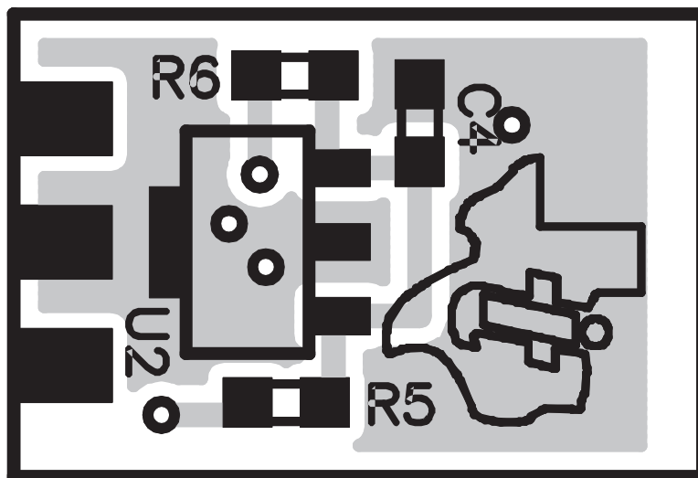
Figure 2–7. Bottom Assembly (Bottom View)
