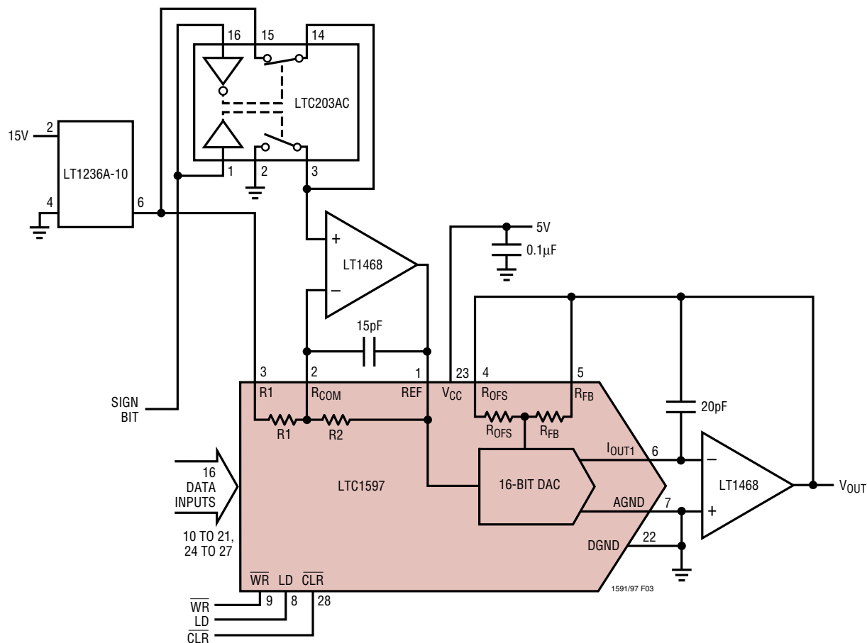
17-Bit Sign Magnitude DAC with Bipolar Zero Error of 140µV (0.92LSB at 17 Bits) at 25°C
