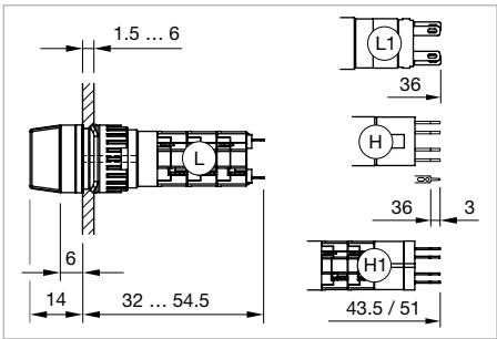
Dimensions [mm] H = Universal terminal 2.0 x 0.5 mm, H1 = Universal-Solder terminal, L = Solder terminal, L1 = Solder terminal 2.8 x 0.5 mm
