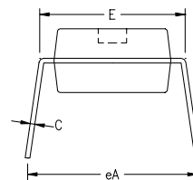
Figure 37. 20-Pin Plastic Dual Inline Package (PDIP)
