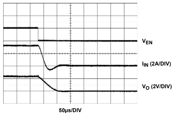
FIGURE 14. SHUT-DOWN
