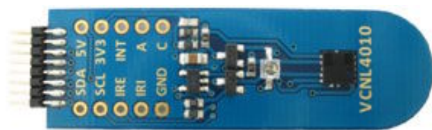
VCNL4010 Sensor Board
