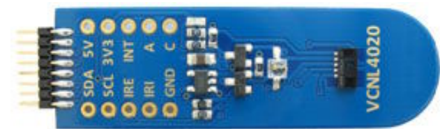
Fig. 5 - VCNL4020 Sensor Board
