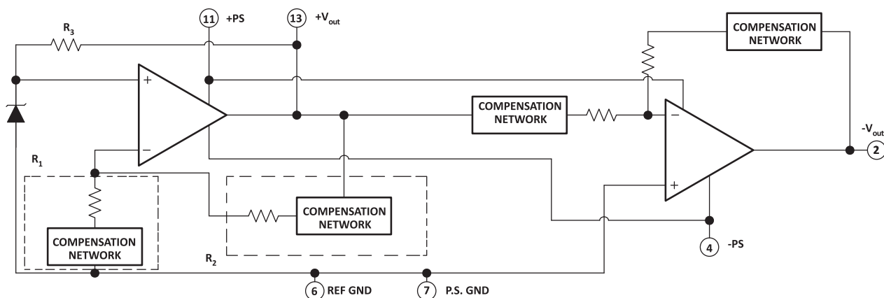
Figure 12: Block Diagram
