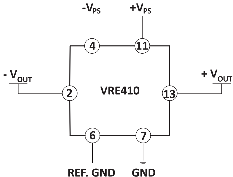
Figure 1: Typical Connection
