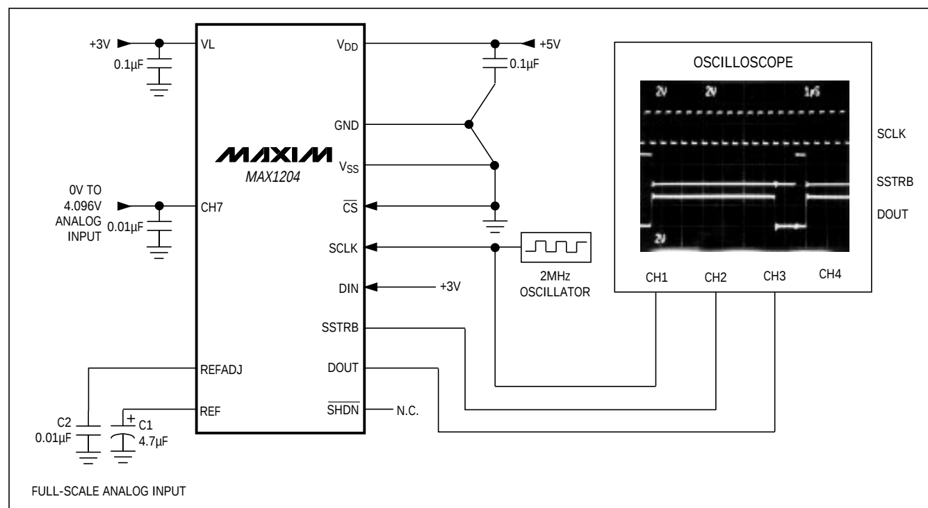
Figure 5. Quick-Look Circuit
