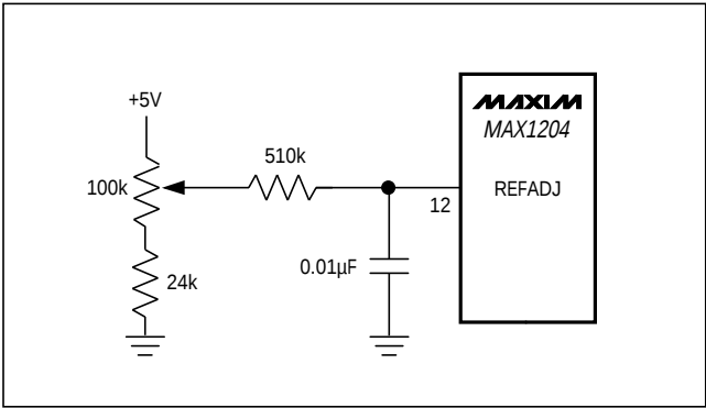
Figure 17. Reference-Adjust Circuit
