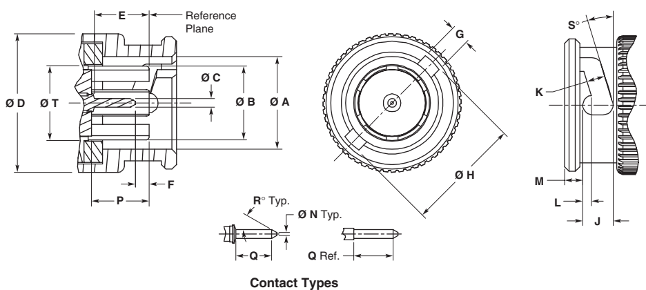
Contact Types
