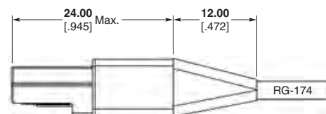
Cable Plug
