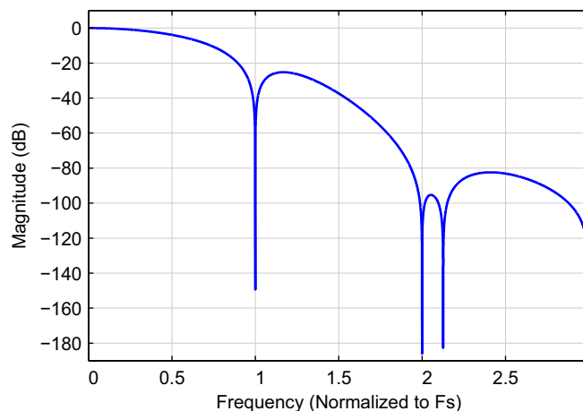
Figure 9-58. Stopband Attenuation
