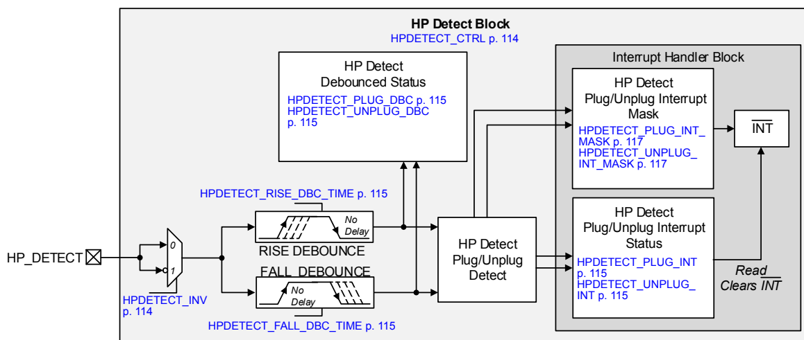
Figure 4-8. Headphone Detect Block Diagram
