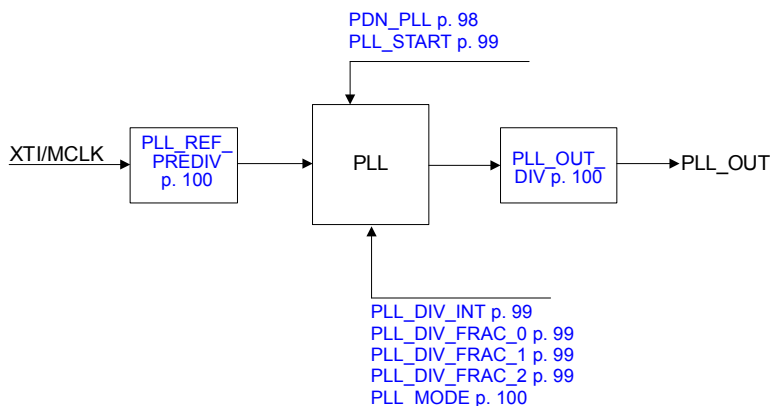
Figure 4-15. Fractional-N PLL
