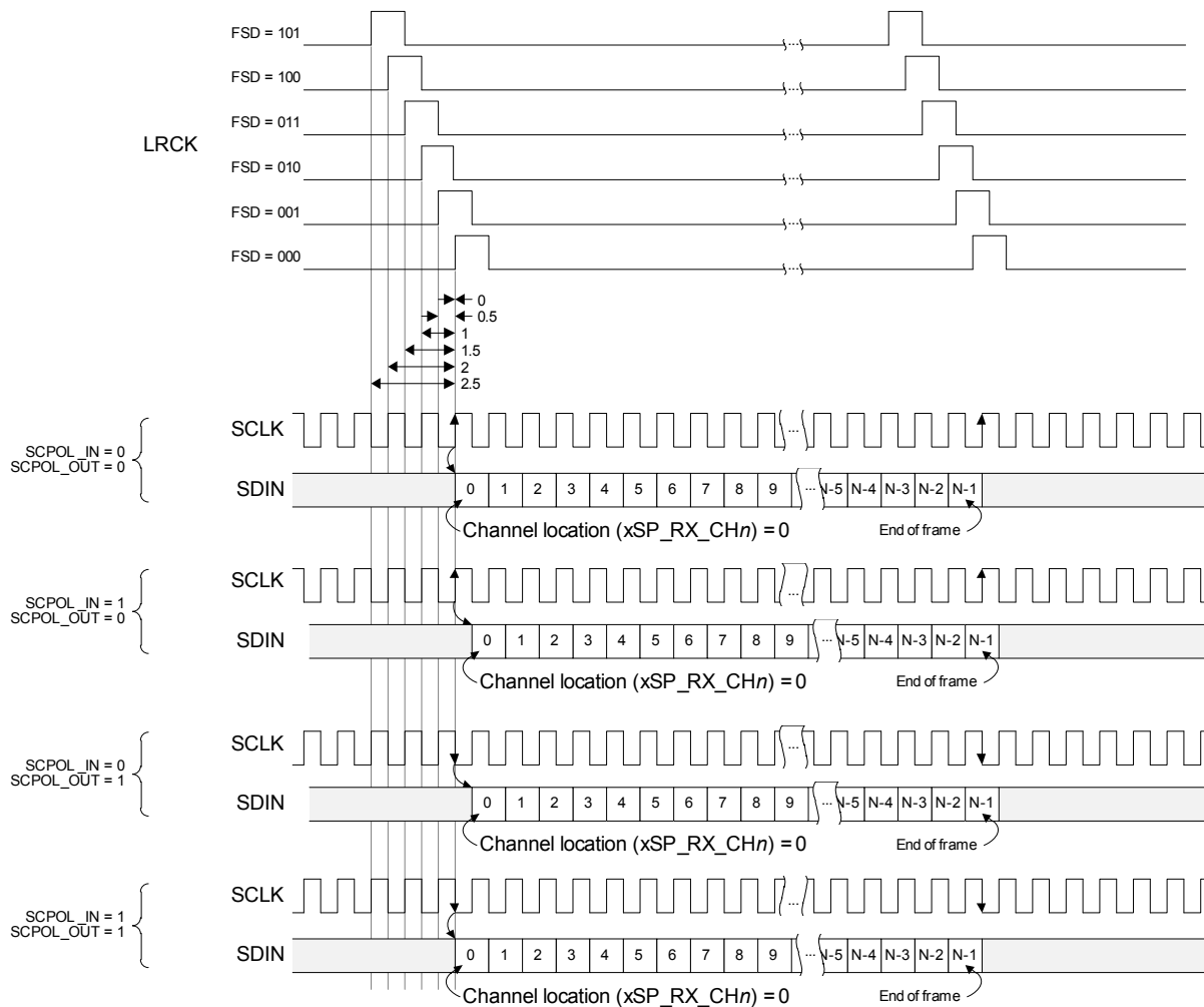
Figure 4-21. LRCK FSD and SCLK Polarity Example Diagram
