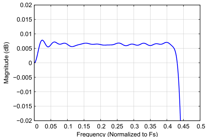
Figure 9-1. Passband Ripple
