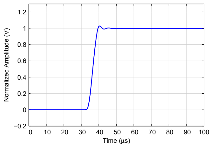
Figure 9-64. Step Response
