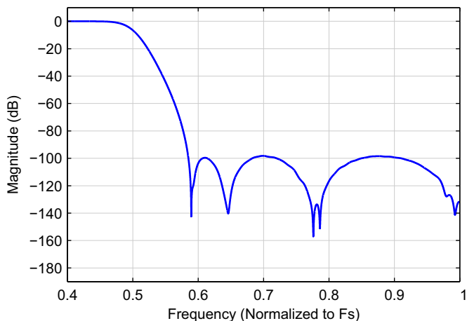
Figure 9-2. Stopband Attenuation
