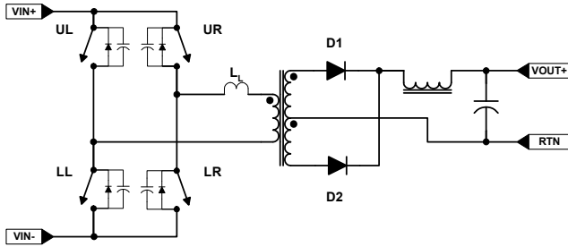
FIGURE 15. IDEALIZED FULL-BRIDGE
