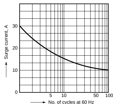
2-1. Surge current and time (OAC)
