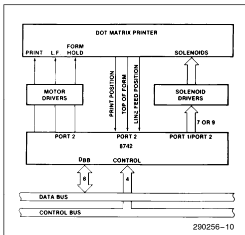
Figure 6. 8742 80-Column Matrix Printer Interface
