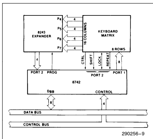
Figure 5. 8742-8243 Keyboard Scanner
