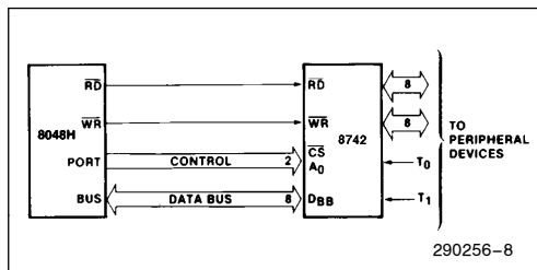
Figure 4. 8048H-8742 Interface
