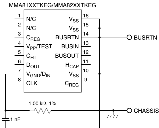
Figure 1-5. V_{GND}/D_{IN} Connection Options
