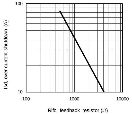
Figure 11 – Ids (A) Vs Rf1b (Ω)
