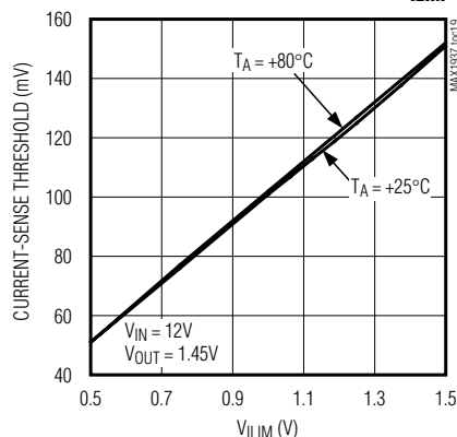
CURRENT-SENSE THRESHOLD vs. V_{ILIM}
