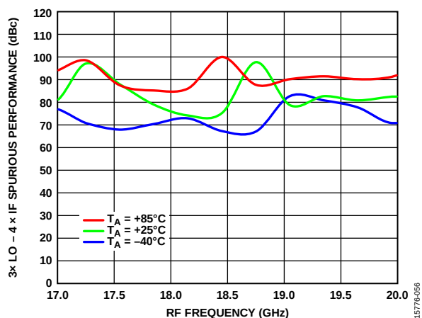
Figure 56. 3 \times \text{LO} - 4 \times \text{IF} Spurious Performance vs. RF Frequency at Various Temperatures, IF Frequency = 3.3 GHz
