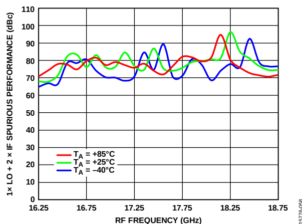
Figure 58. 1 \times \text{LO} + 2 \times \text{IF} Spurious Performance vs. RF Frequency at Various Temperatures
