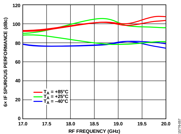
Figure 57. 6 \times \text{IF} Spurious Performance vs. RF Frequency at Various Temperatures, RF Frequency = 18 GHz
