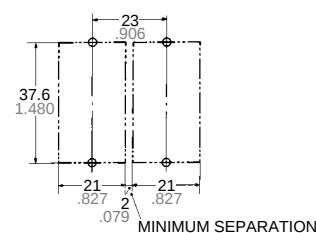
CHASSIS CUTOUT IN TANDEM MOUNTING
