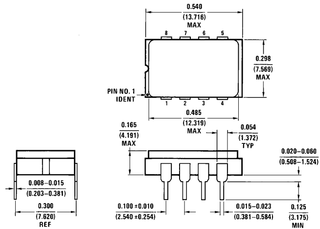
8-Pin Ceramic Sidebraced Dual-In-Line Package Order Number LM6142AMJ/883 NS Package Number D08C
