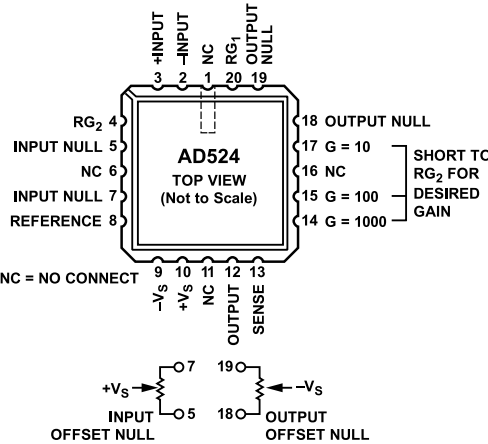
Figure 4. Leadless Chip Carrier (E)
