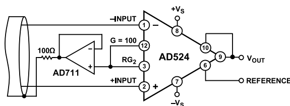
Figure 41. Shield Driver, G \geq 100
