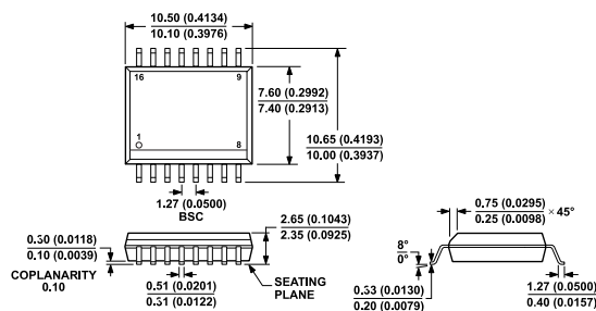
Figure 57. 16-Lead Standard Small Outline Package [SOIC_W] Wide Body (RW-16)
