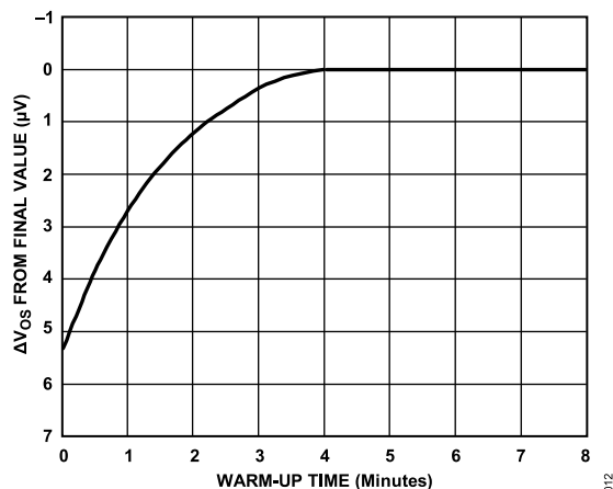
Figure 12. Offset Voltage, RTI, Turn-On Drift
