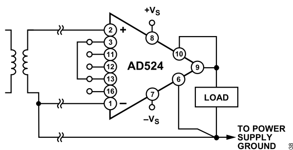
Figure 38. Indirect Ground Returns for Bias Currents—Transformer Coupled
