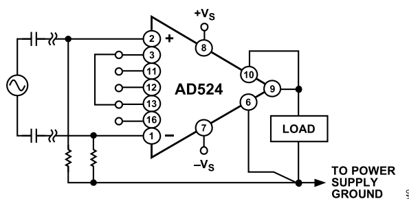
Figure 40. Indirect Ground Returns for Bias Currents—AC-Coupled
