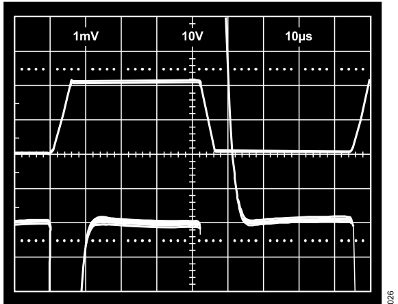
Figure 28. Large Signal Pulse Response and Settling Time, Gain = 10
