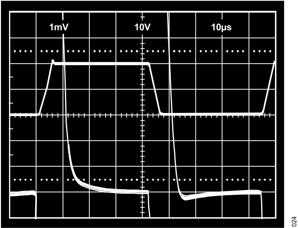
Figure 27. Large Signal Pulse Response and Settling Time, Gain = 1
