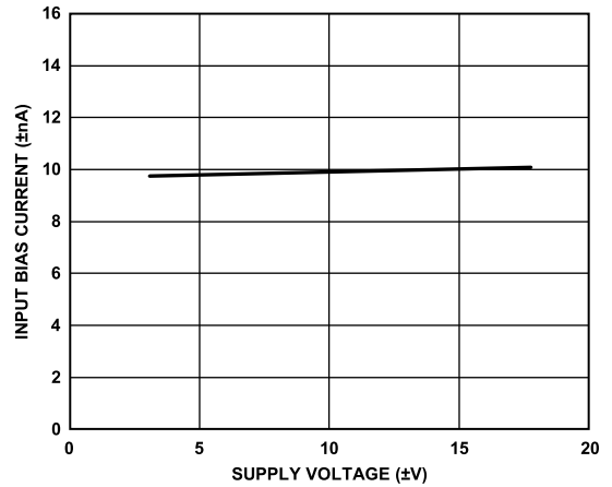
Figure 9. Input Bias Current vs. Supply Voltage
