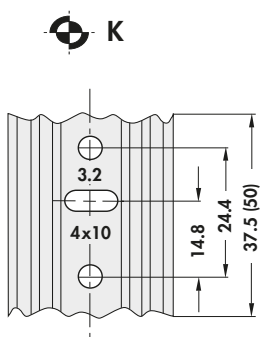
SOT 32 / TO 220 exceeding \geq 37.5 mm
