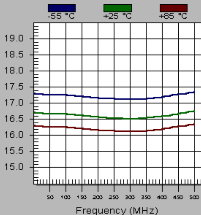
TM6511 Gain (dB)
