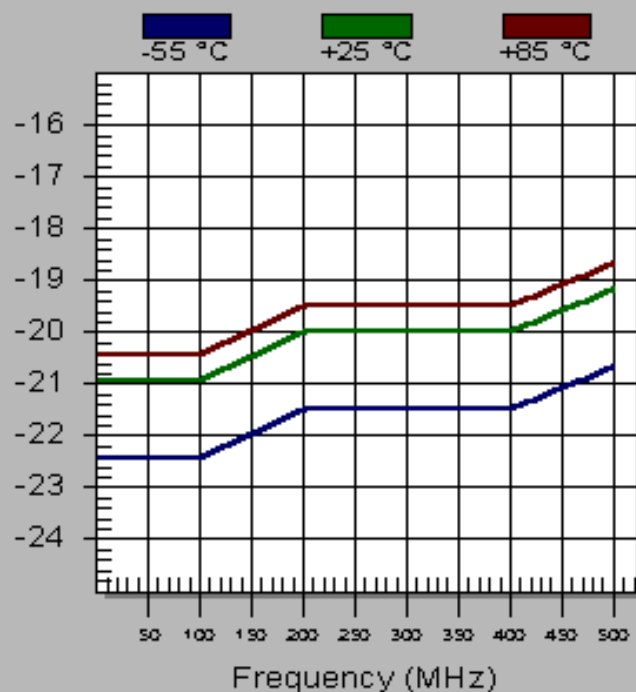
TM6511 Reverse Isolation (dB)
