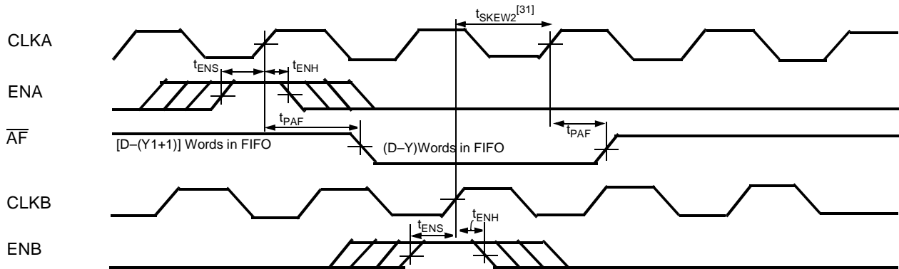
Timing for \overline{AF} when FIFO is Almost Full (CY Standard and FWFT Modes) [28, 29, 30, 35]
