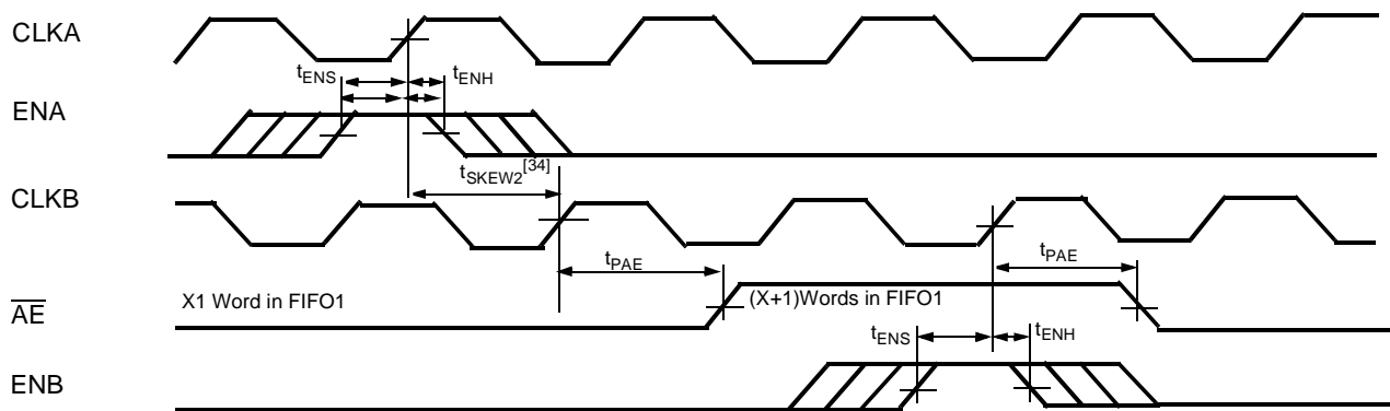
Timing for \overline{AE} when FIFO is Almost Empty (CY Standard and FWFT Modes) [32, 33, 35]
