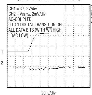
DIGITAL FEEDTHROUGH GLITCH IMPULSE (0 TO 1 DIGITAL TRANSITION)
